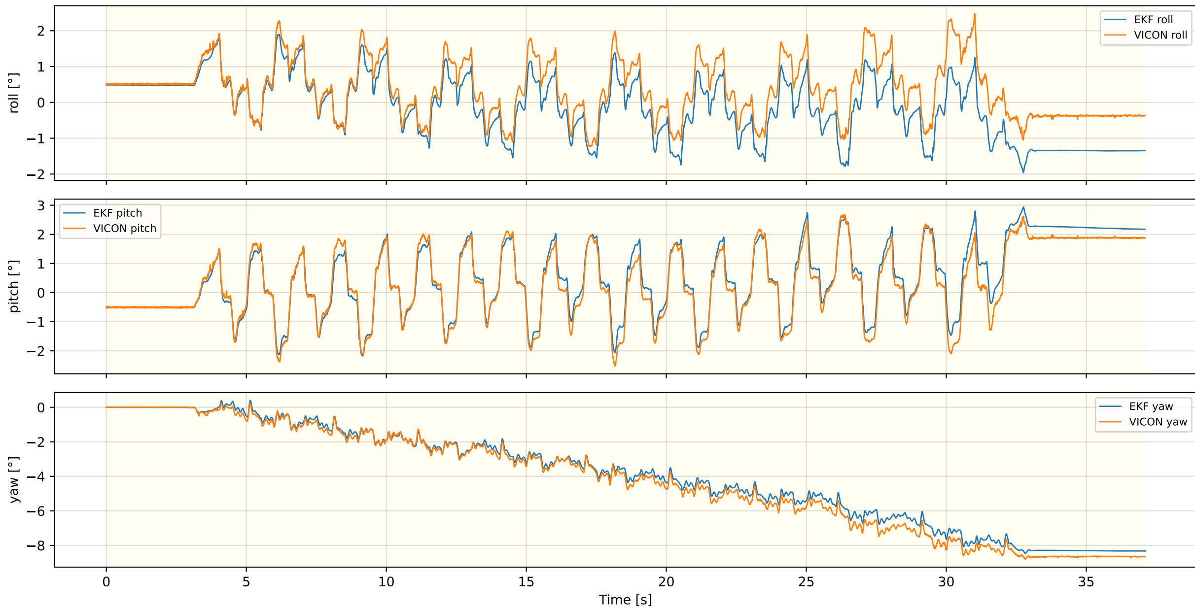
Inner EKF Attitude — FLAT_WLW_NEW_REAL_3
