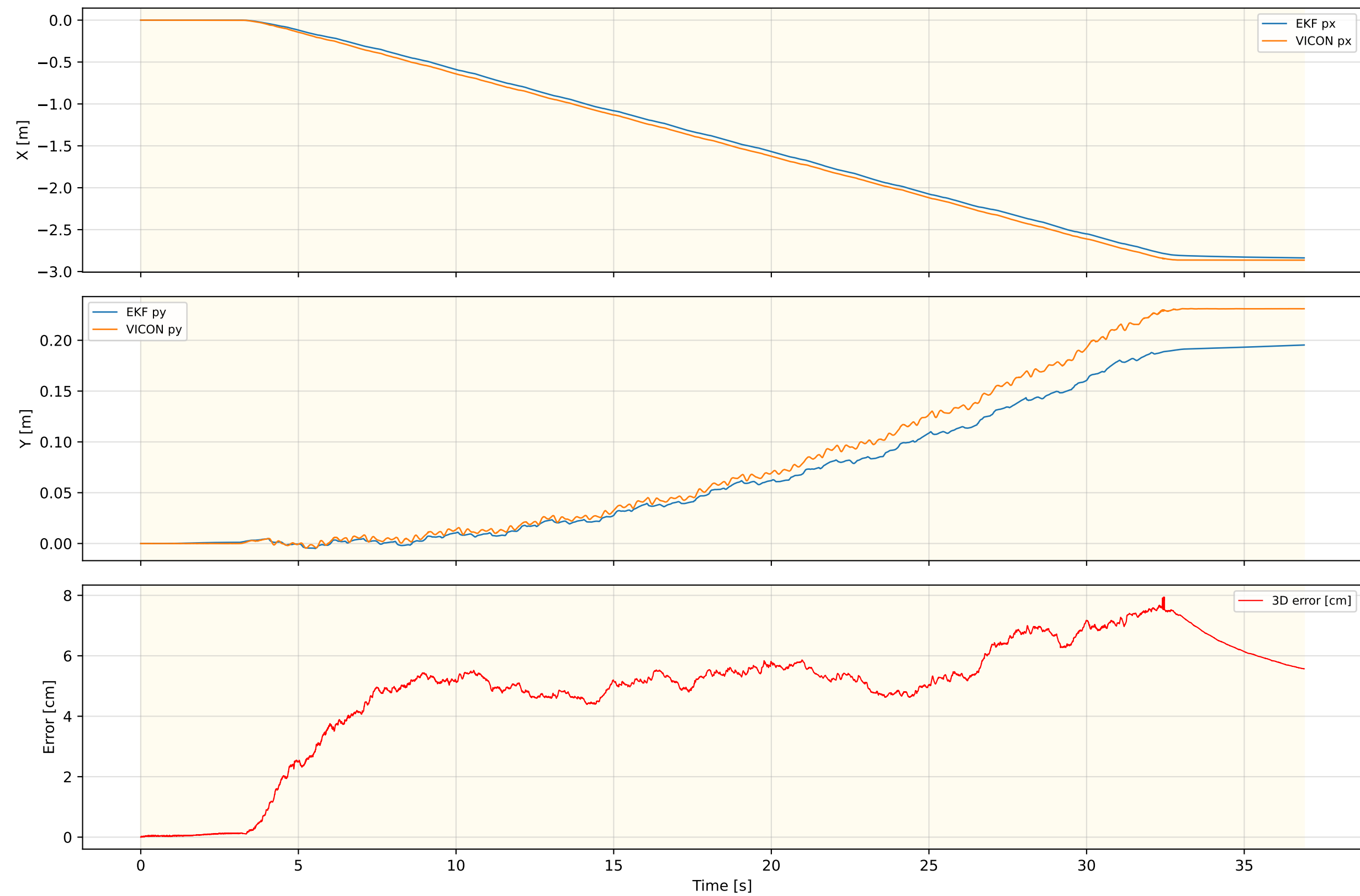
Inner EKF Position — FLAT_WLW_NEW_REAL_5
