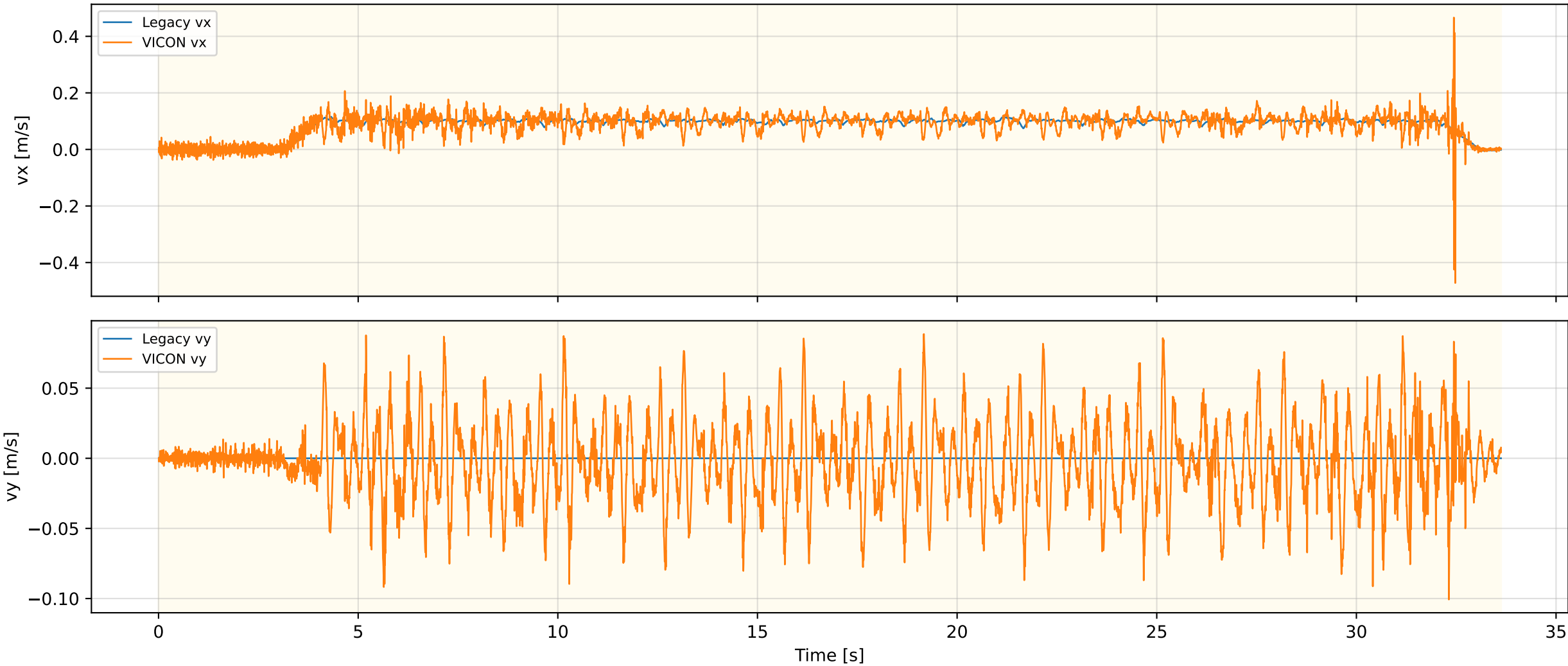
Legacy Odometry Velocity — FLAT_WLW_OLD_REAL_1
