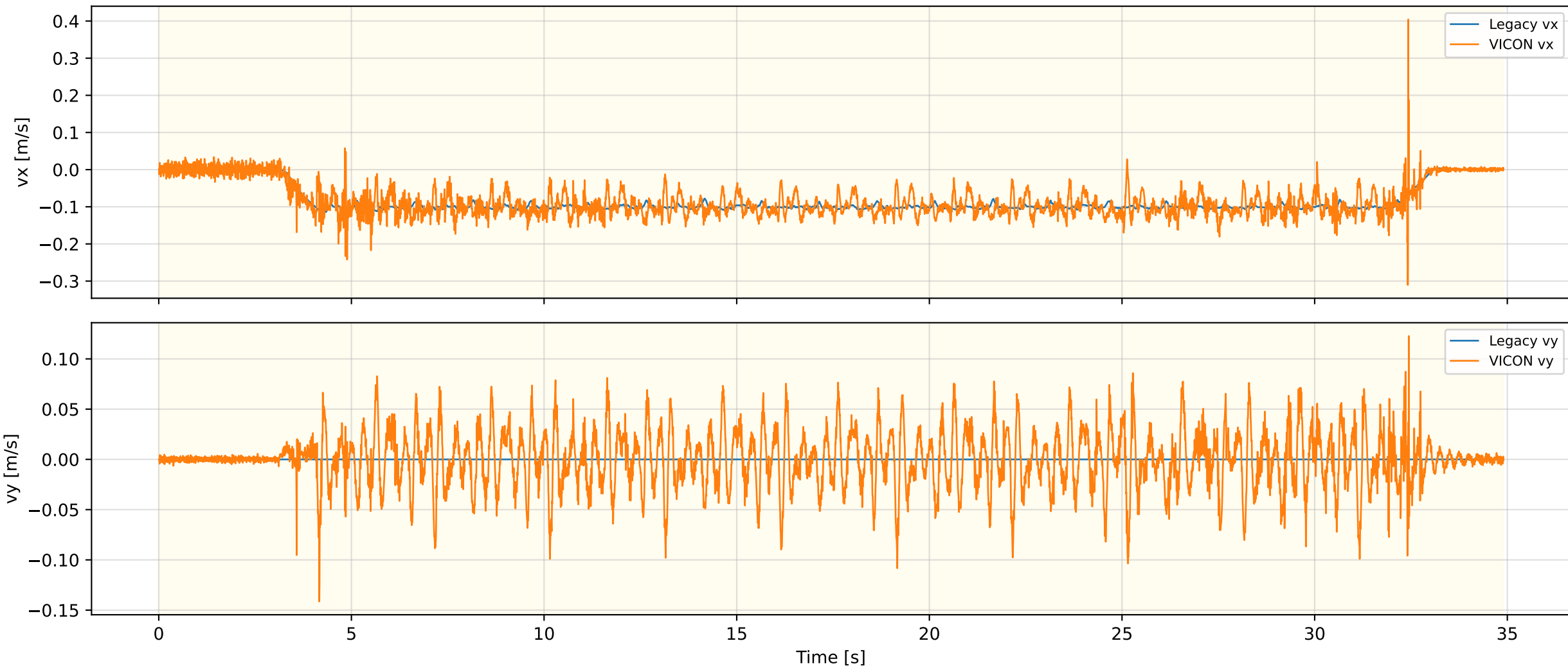
Legacy Odometry Velocity — FLAT_WLW_OLD_REAL_3
