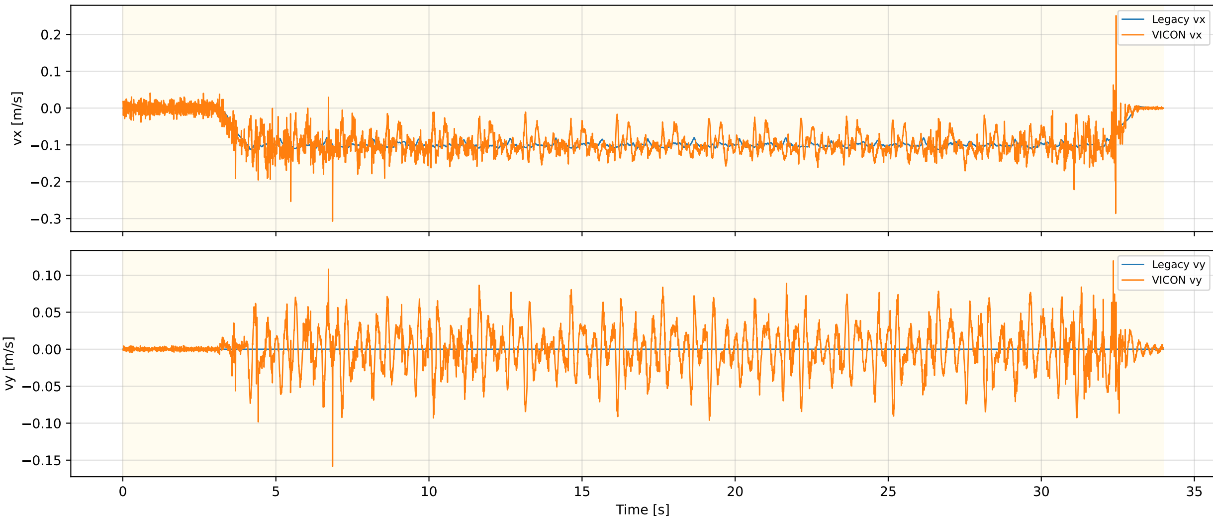
Legacy Odometry Velocity — FLAT_WLW_OLD_REAL_4
