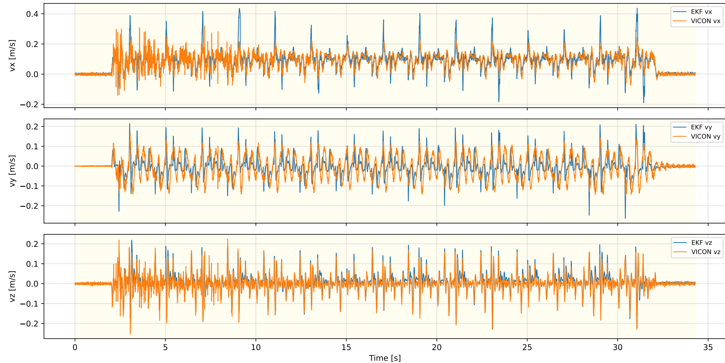
Inner EKF Velocity — FLAT_Walk_NEW_REAL_5
