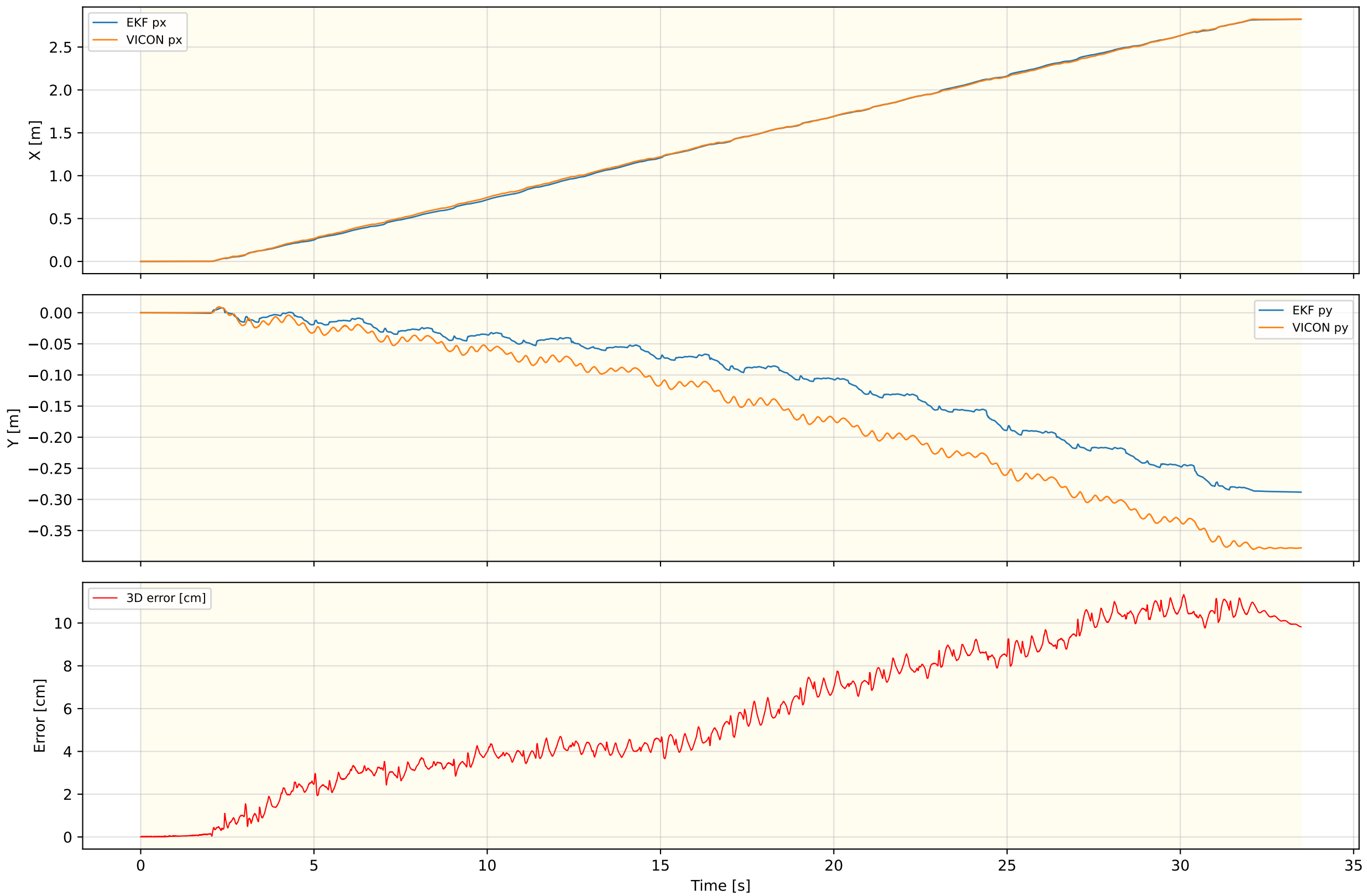
Inner EKF Position — FLAT_Walk_NEW_REAL_6
