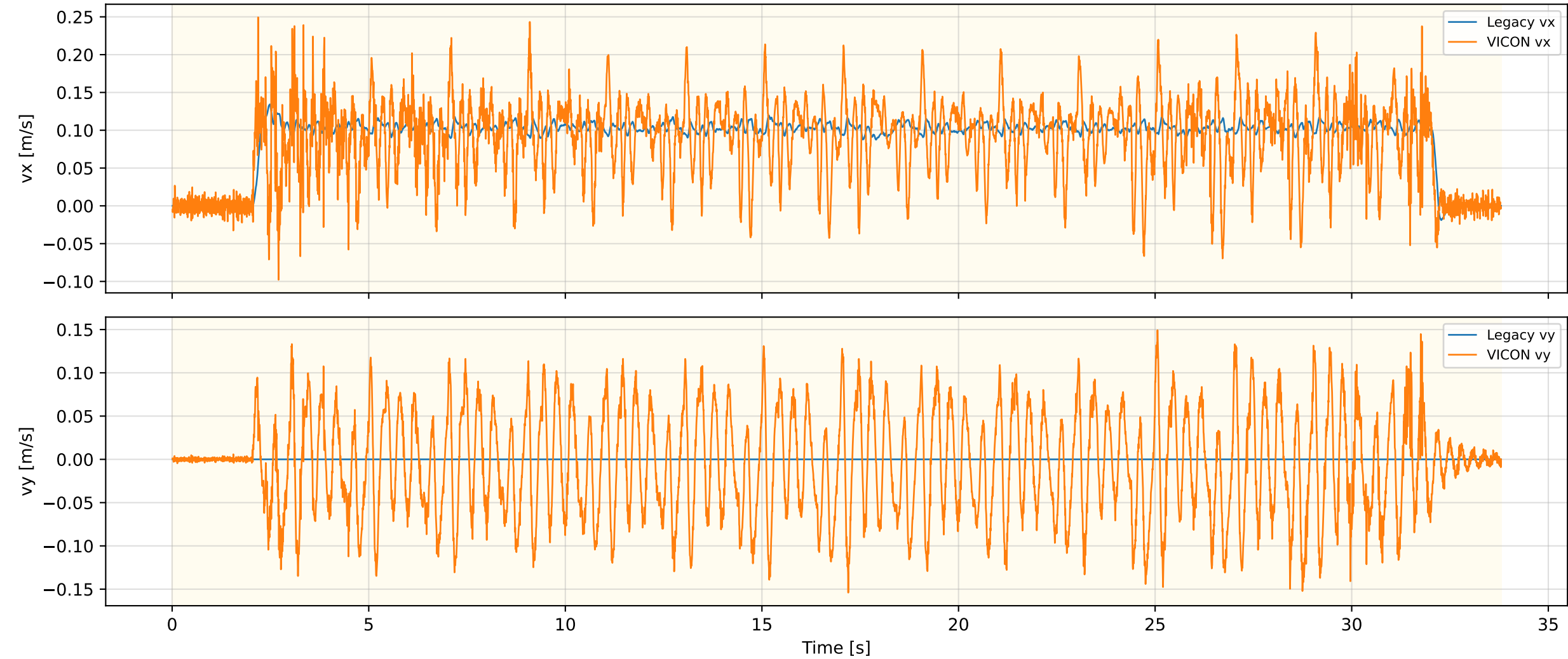
Legacy Odometry Velocity — FLAT_Walk_OLD_REAL_2
