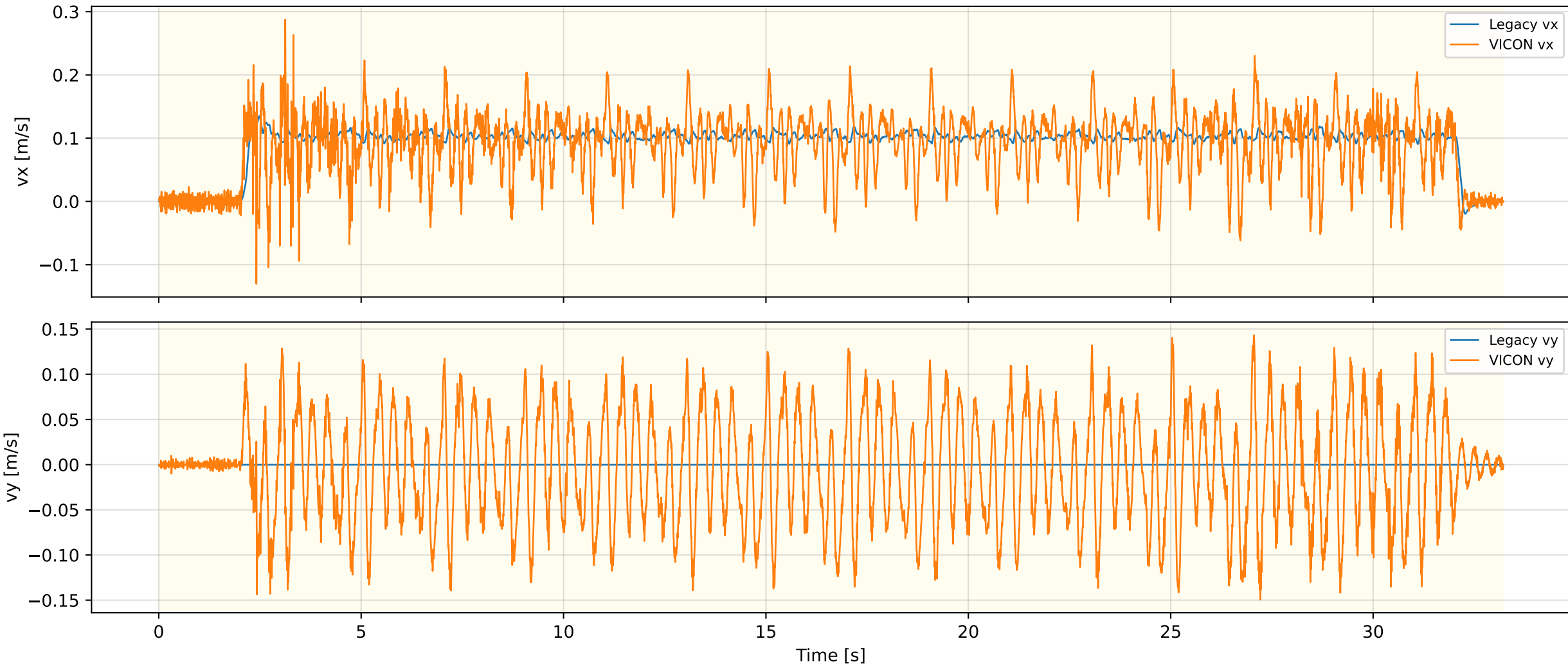
Legacy Odometry Velocity — FLAT_Walk_OLD_REAL_3
