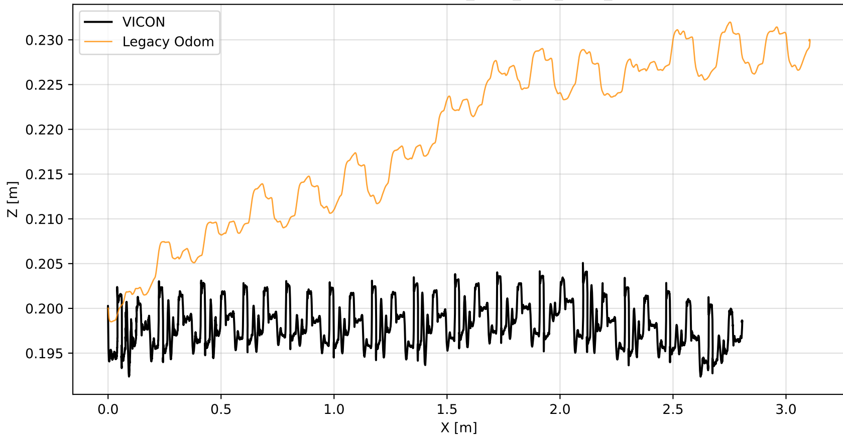
XZ Trajectory — FLAT_Walk_OLD_REAL_5
