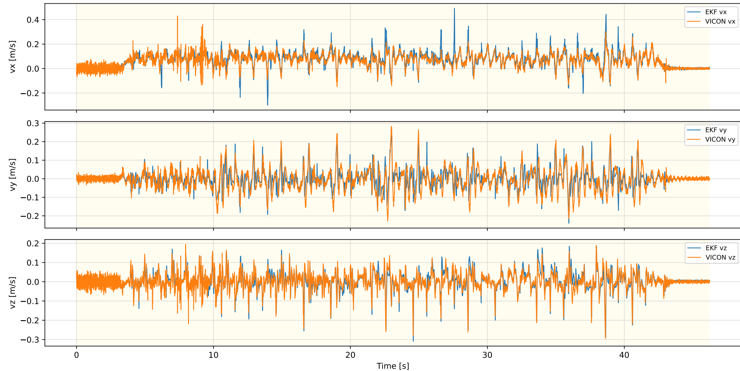
Inner EKF Velocity — OBS_MPC_NEW_REAL_3
