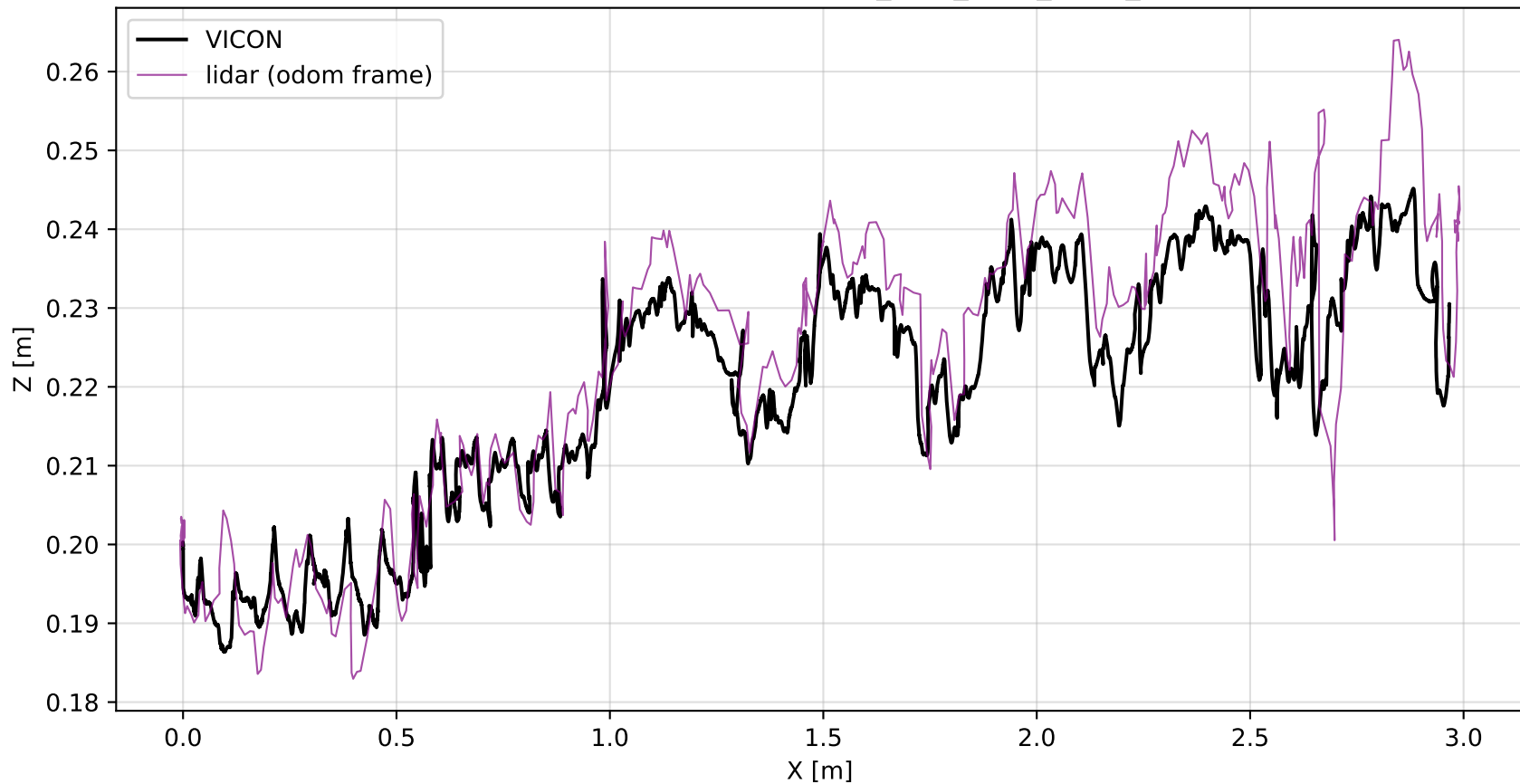
LiDAR XZ Trajectory — OBS_MPC_NEW_REAL_4
