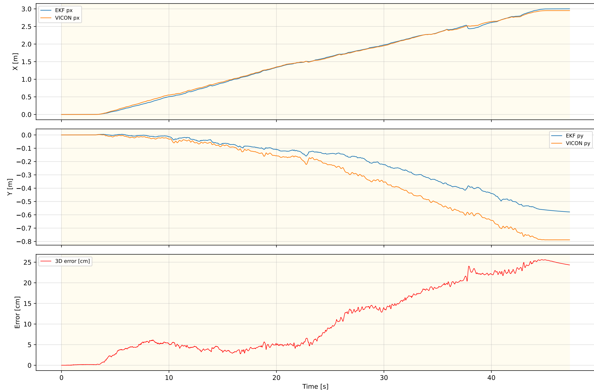
Inner EKF Position — OBS_MPC_NEW_REAL_5
