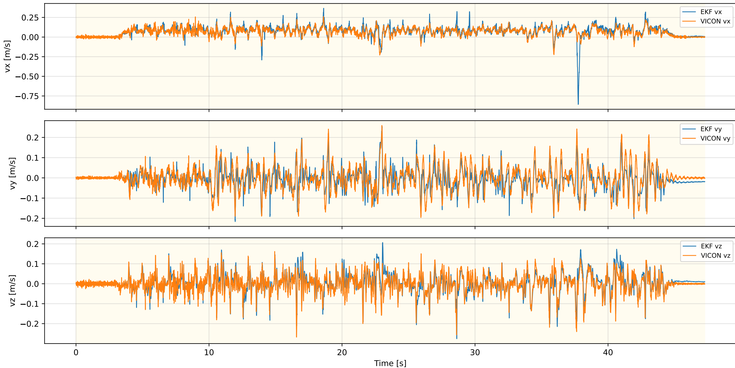
Inner EKF Velocity — OBS_MPC_NEW_REAL_5
