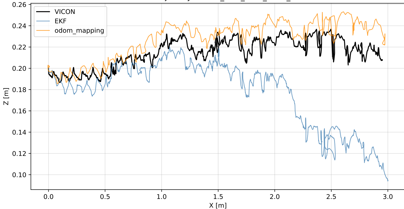
XZ Trajectory — OBS_MPC_NEW_REAL_5
