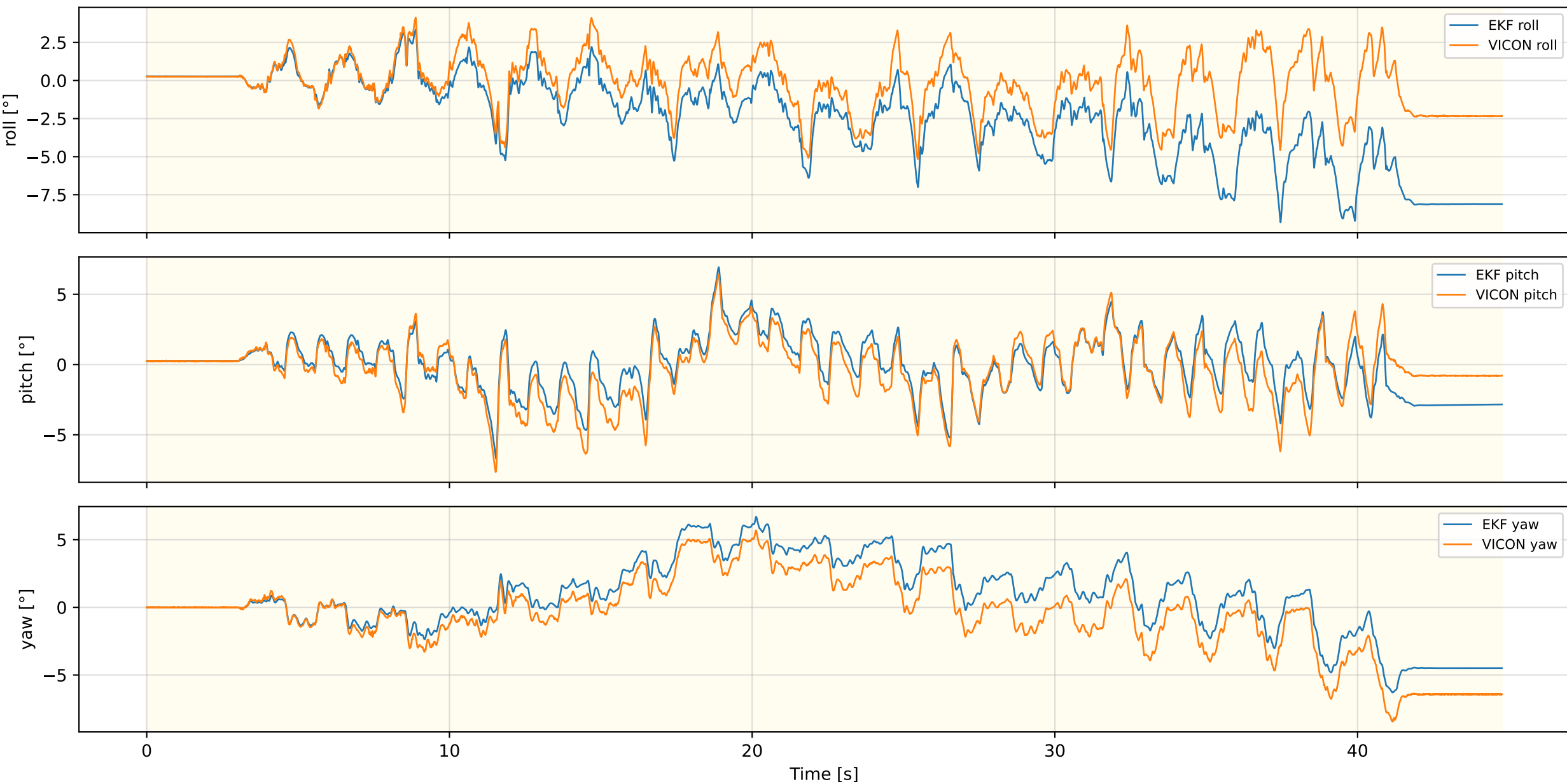
Inner EKF Attitude — OBS_MPC_NEW_REAL_6
