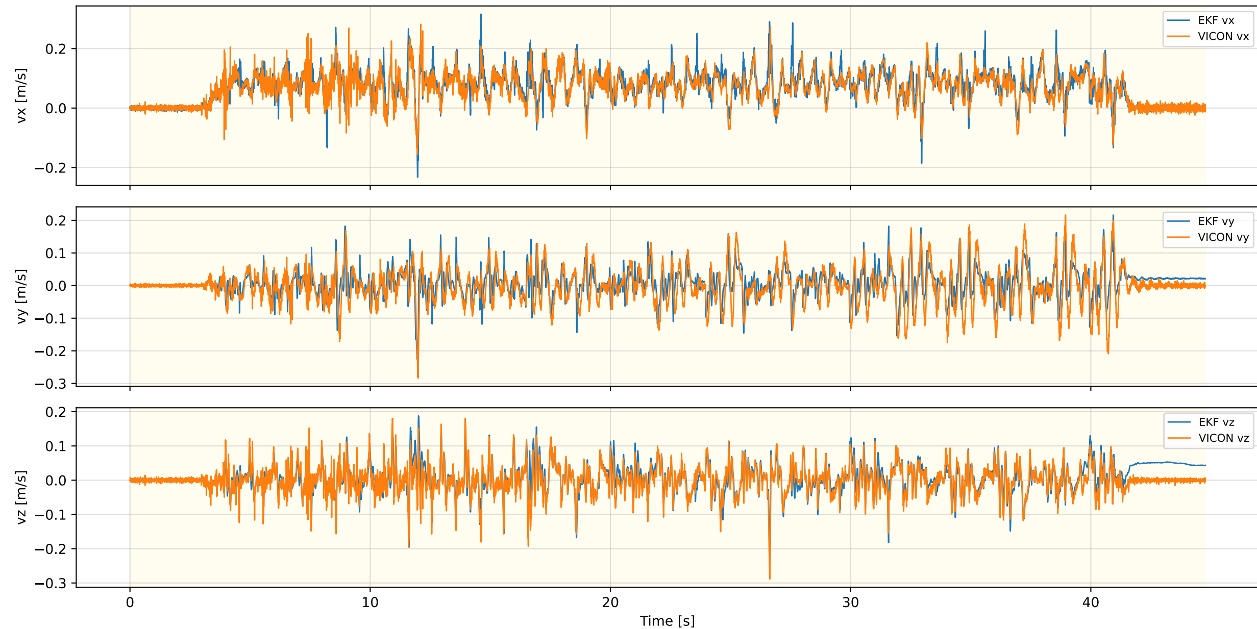
Inner EKF Velocity — OBS_MPC_NEW_REAL_6
