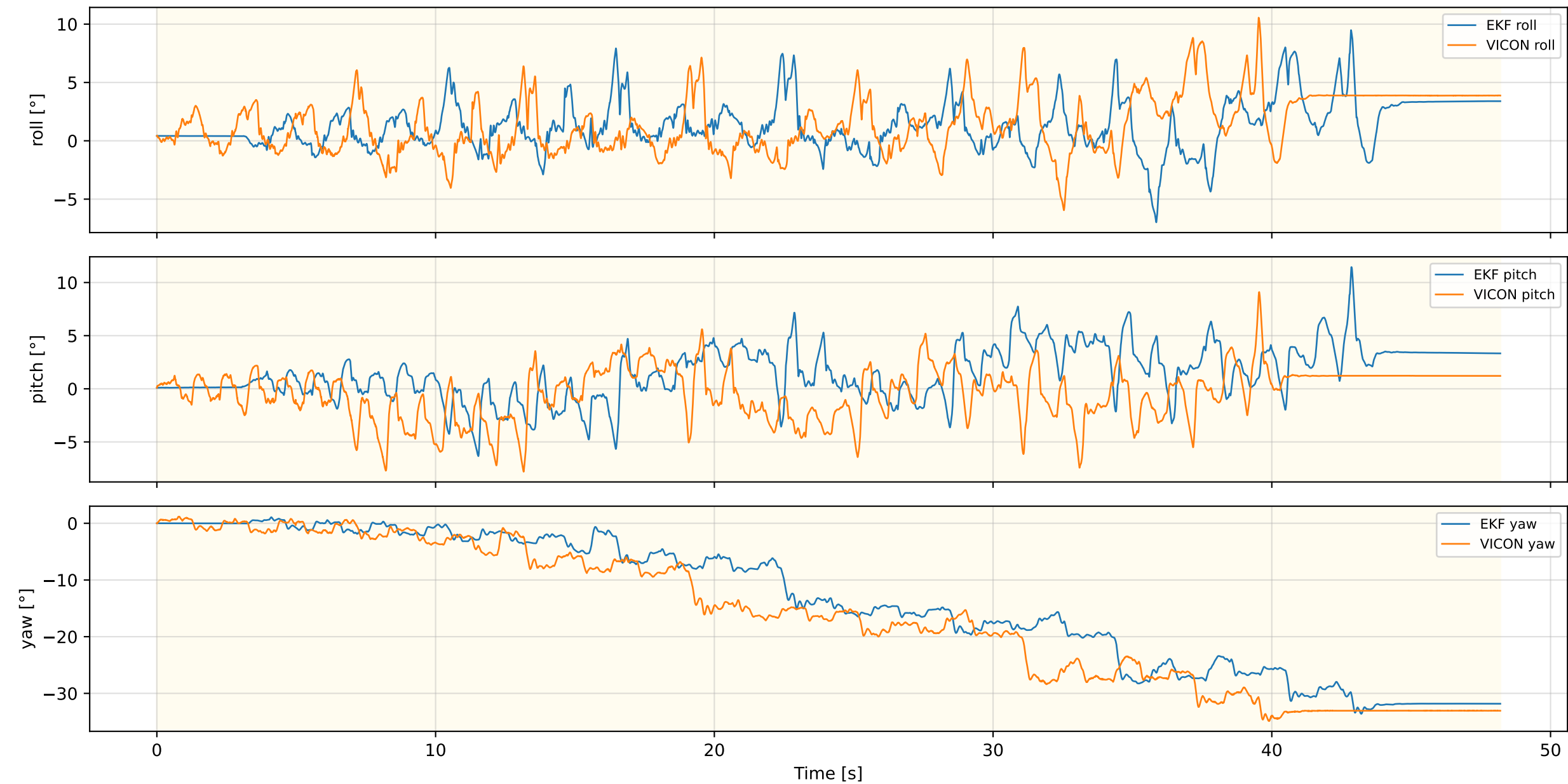
Inner EKF Attitude — OBS_MPC_NEW_REAL_7
