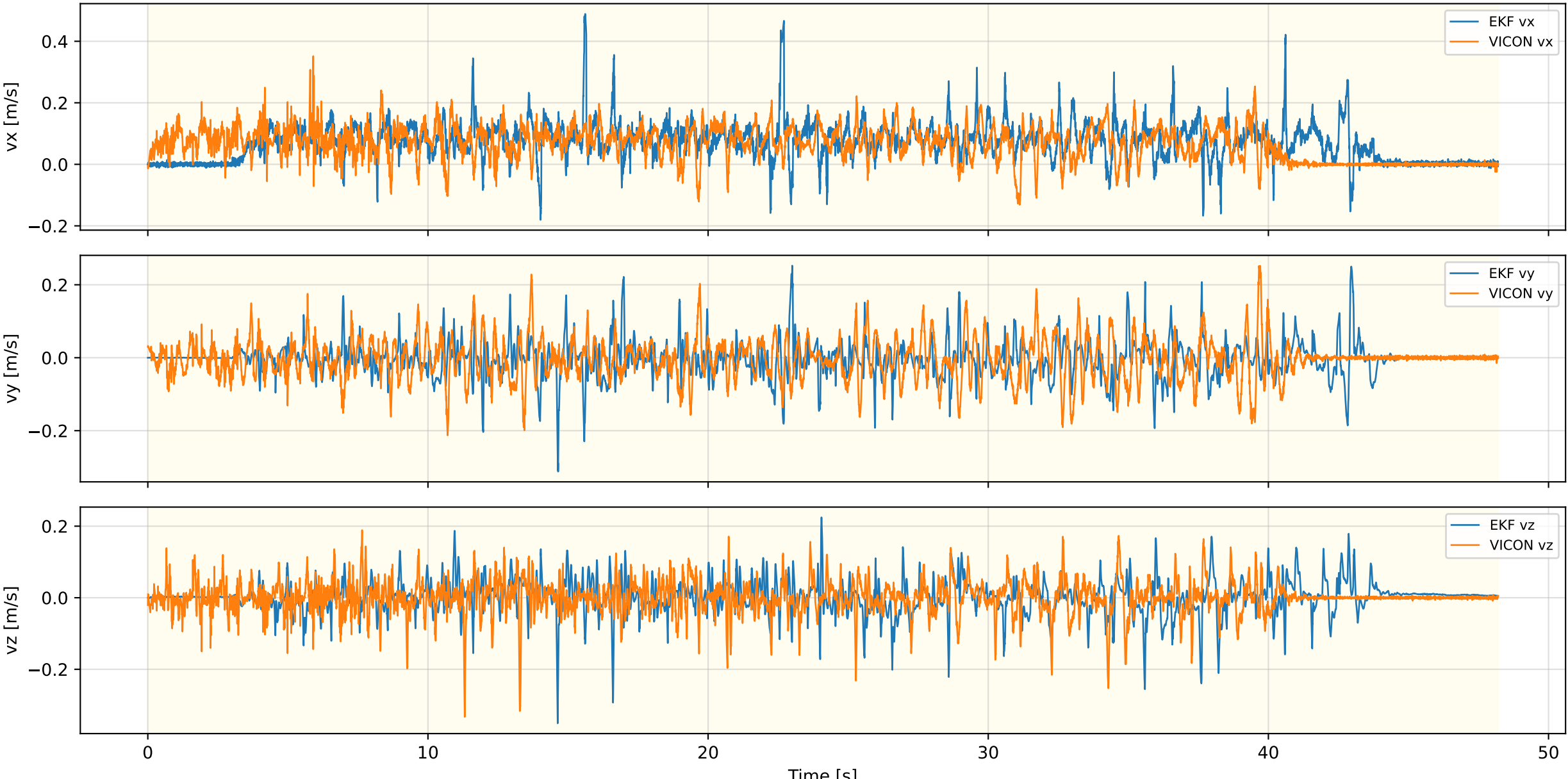
Inner EKF Velocity — OBS MPC NEW REAL 7
