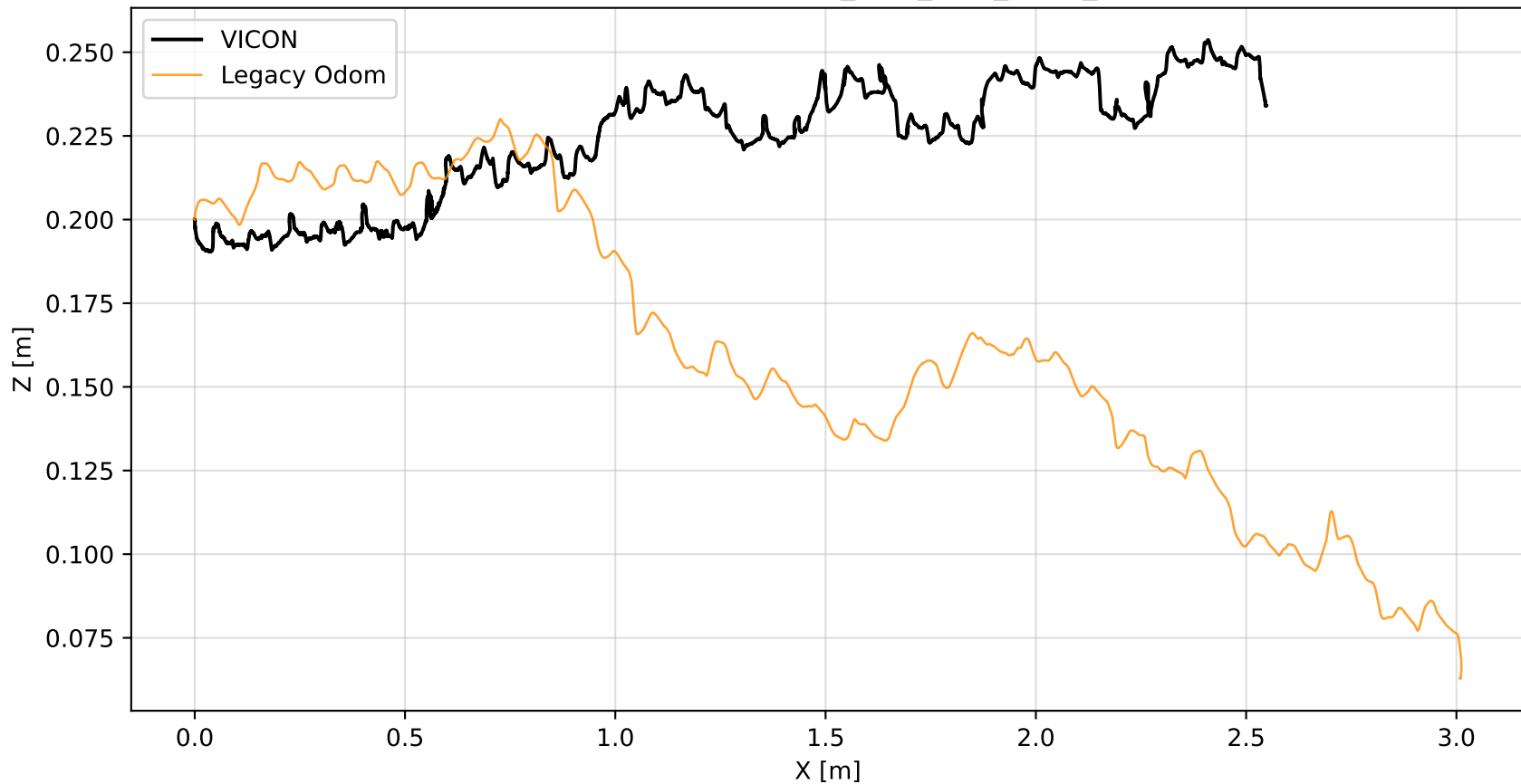
XZ Trajectory — OBS_MPC_OLD_REAL_1
