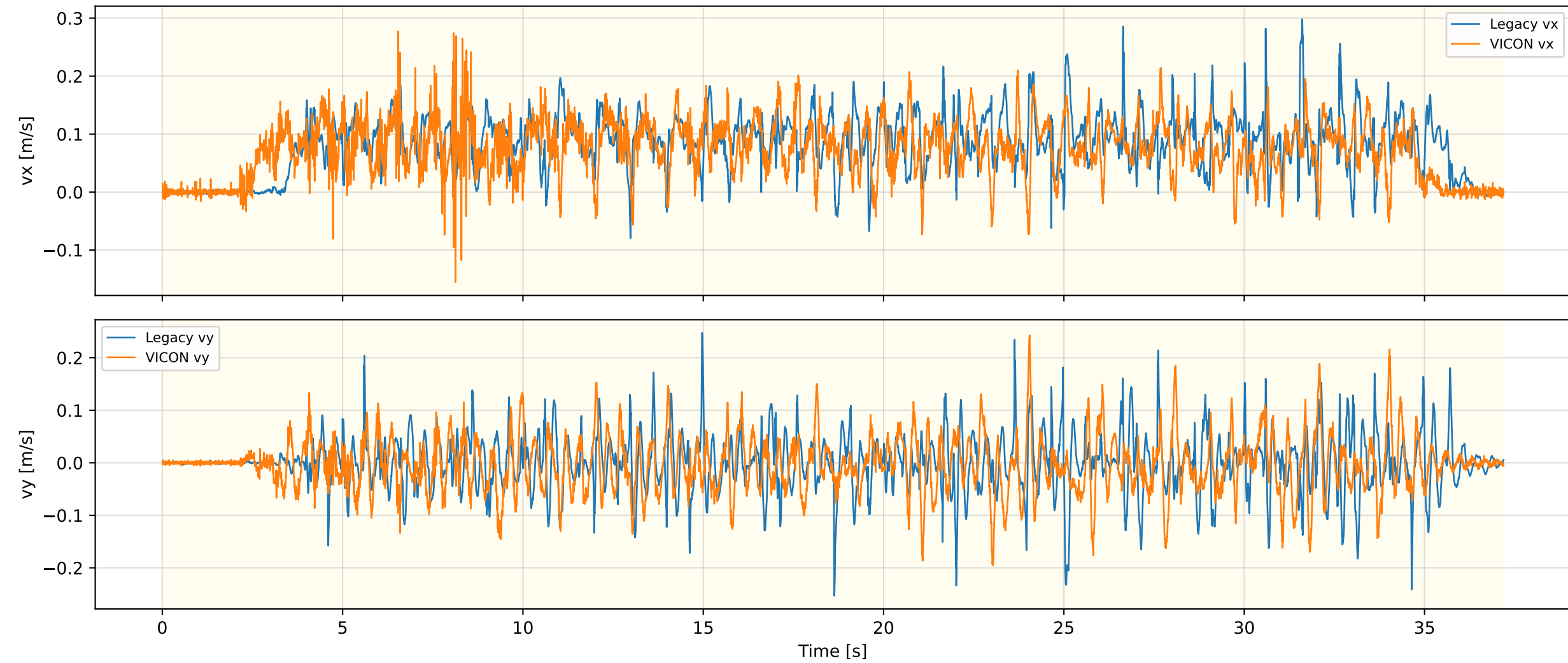
Legacy Odometry Velocity — OBS_MPC_OLD_REAL_3
