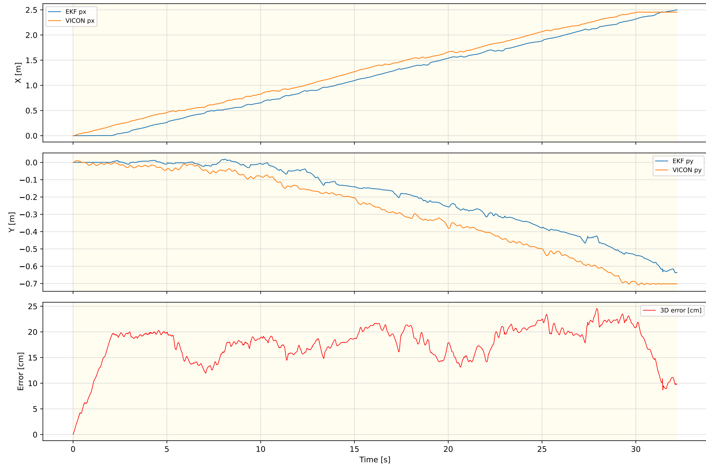
Inner EKF Position — RUGG_Walk_NEW_REAL_1
