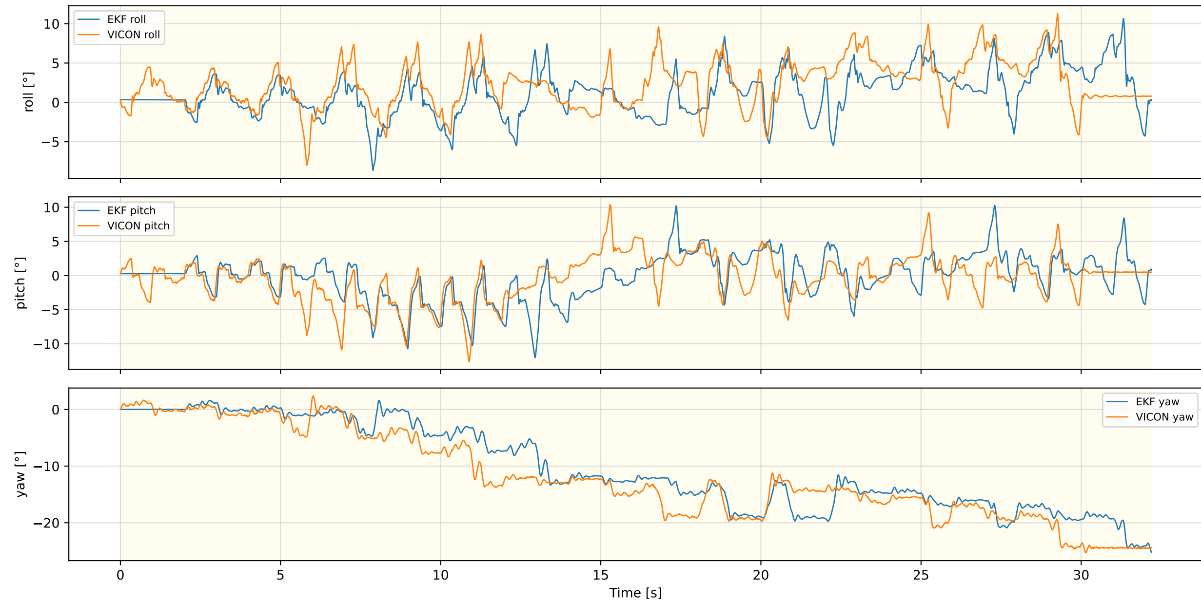
Inner EKF Attitude — RUGG_Walk_NEW_REAL_1
