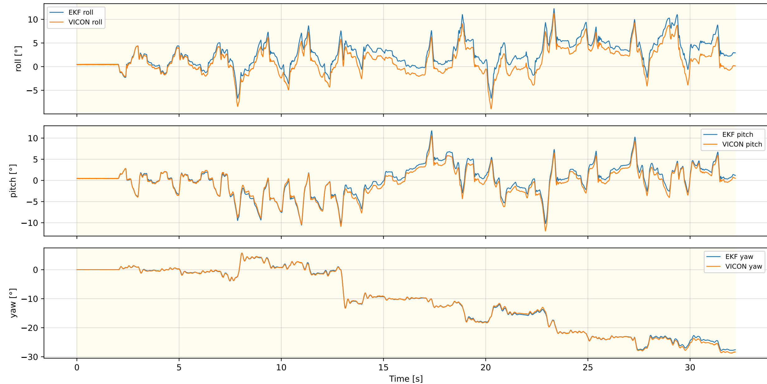
Inner EKF Attitude — RUGG_Walk_NEW_REAL_2
