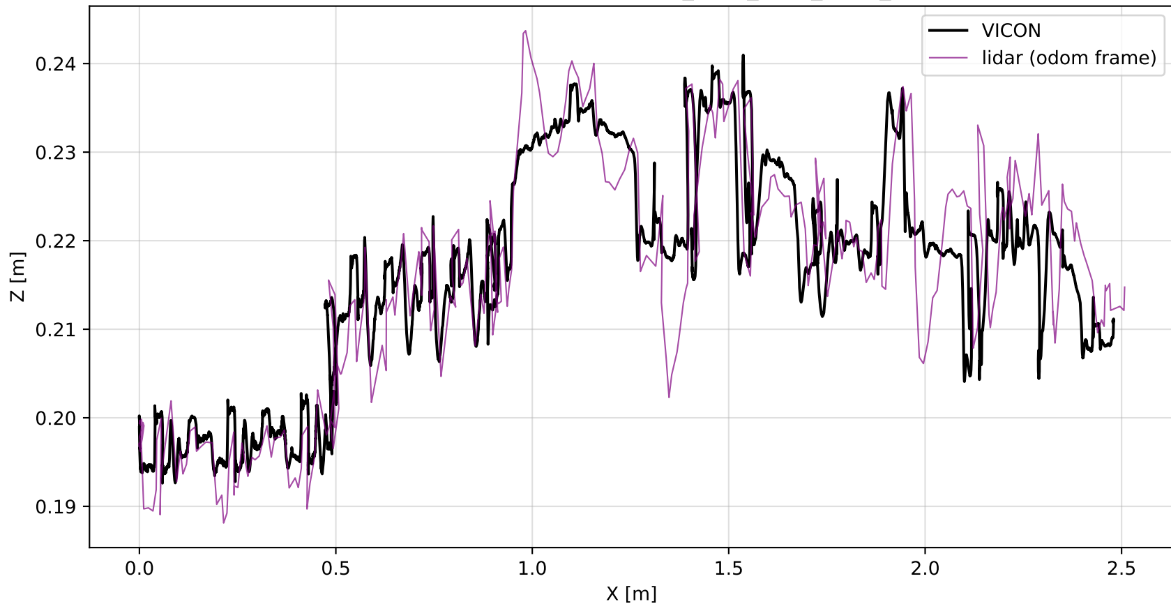
LiDAR XZ Trajectory — RUGG_Walk_NEW_REAL_2
