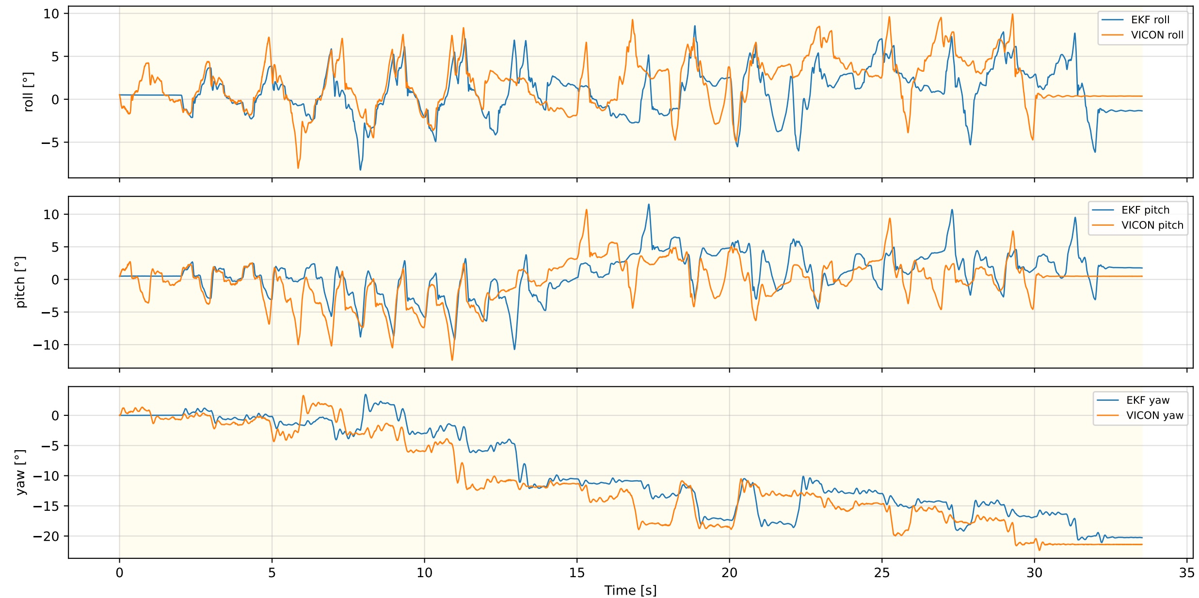
Inner EKF Attitude — RUGG_Walk_NEW_REAL_3
