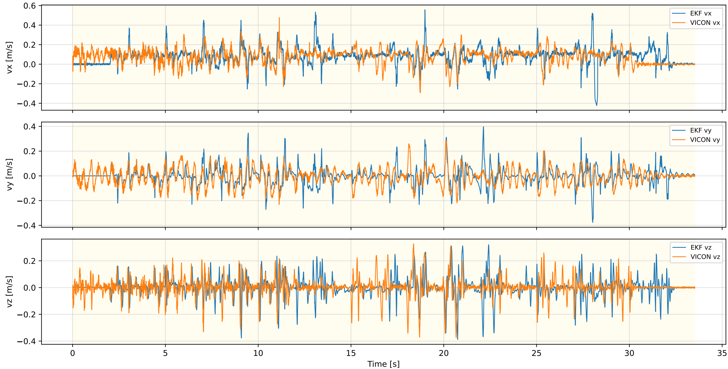
Inner EKF Velocity — RUGG_Walk_NEW_REAL_3
