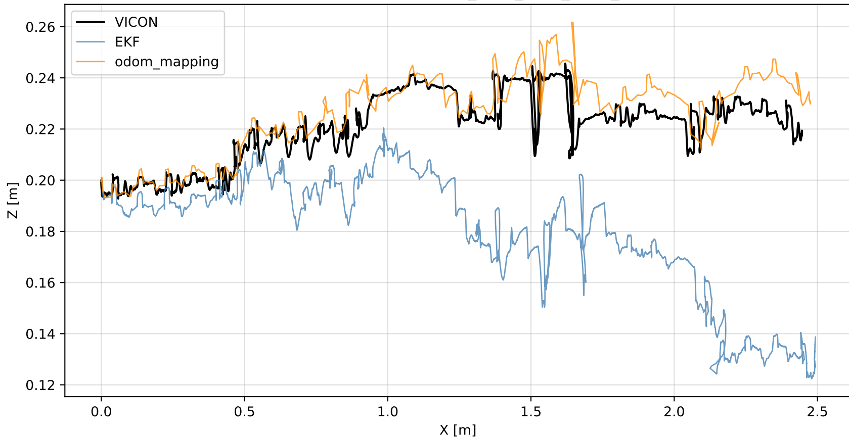
XZ Trajectory — RUGG_Walk_NEW_REAL_3
