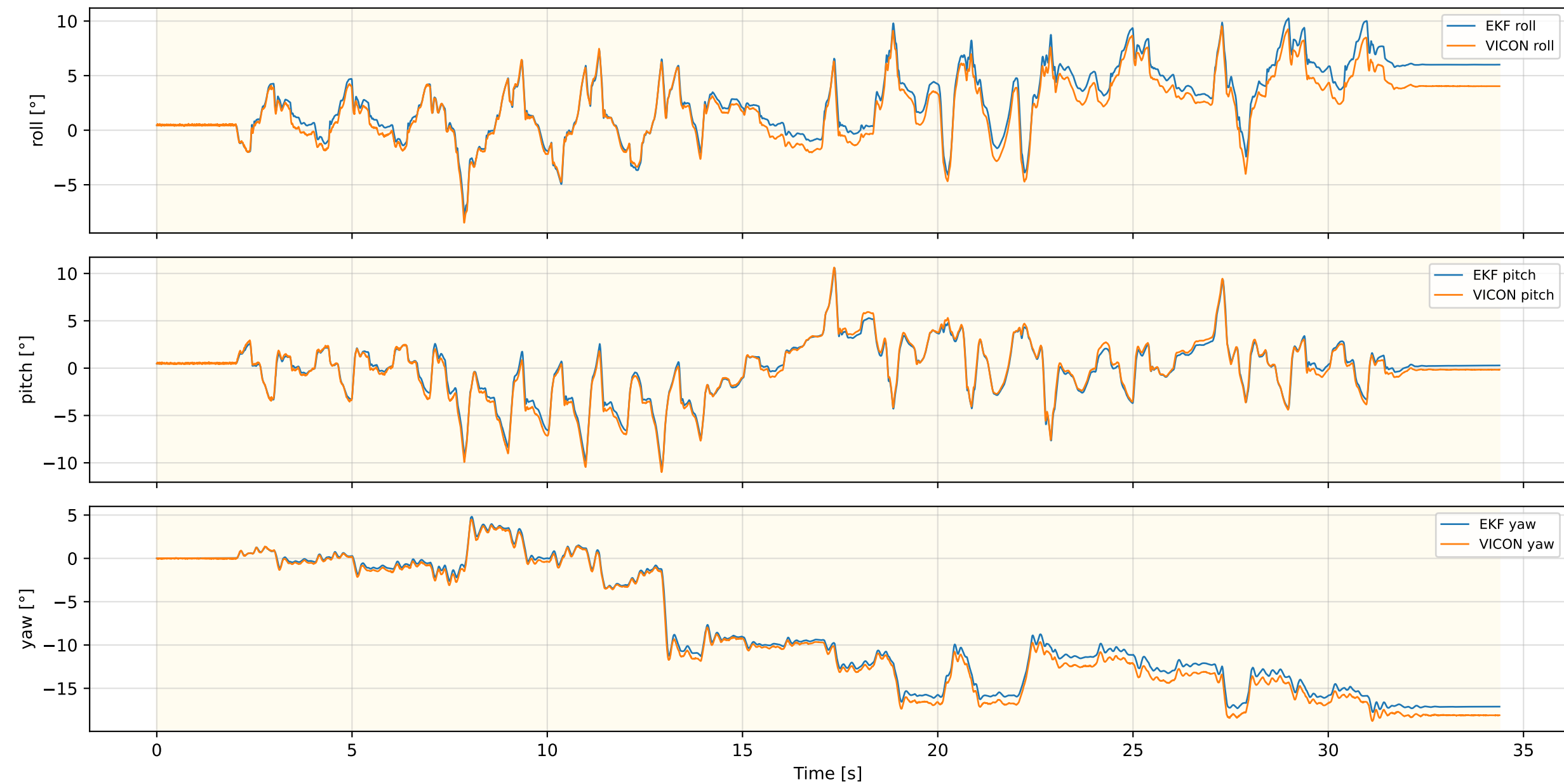
Inner EKF Attitude — RUGG_Walk_NEW_REAL_5
