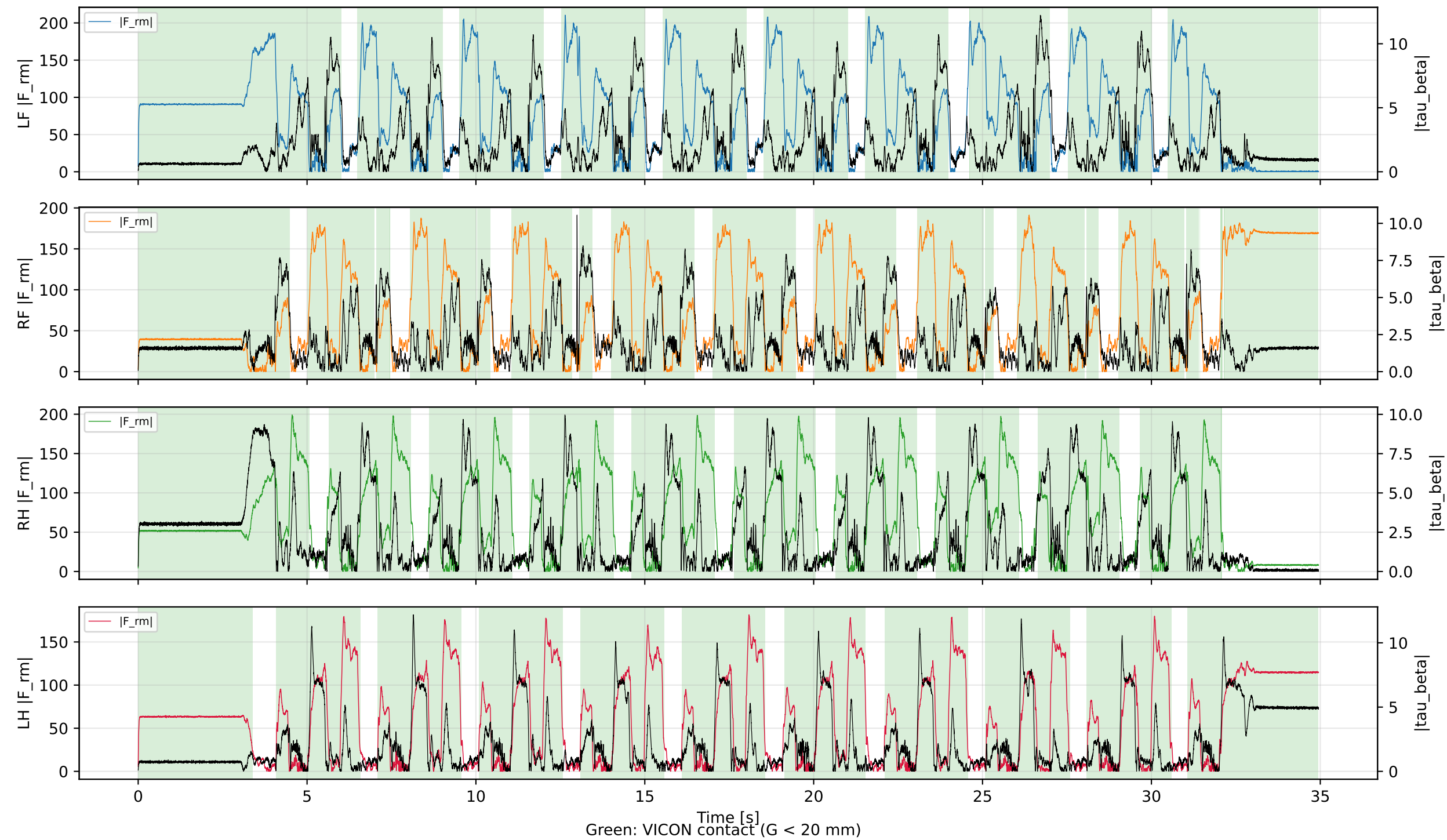
GMO Residuals vs VICON Ground Truth — FLAT_WLW_NEW_REAL_2
