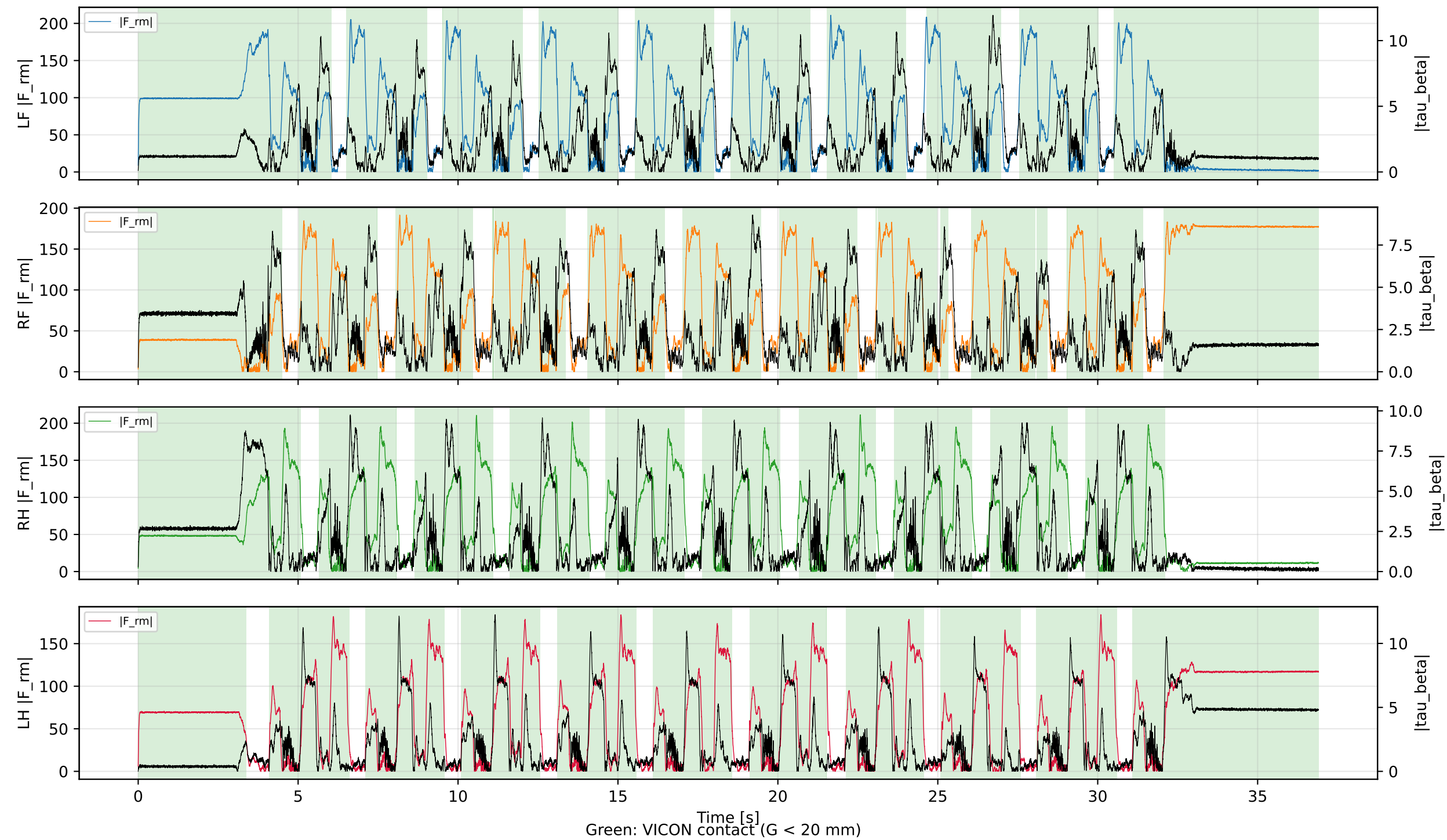
GMO Residuals vs VICON Ground Truth — FLAT_WLW_NEW_REAL_5
