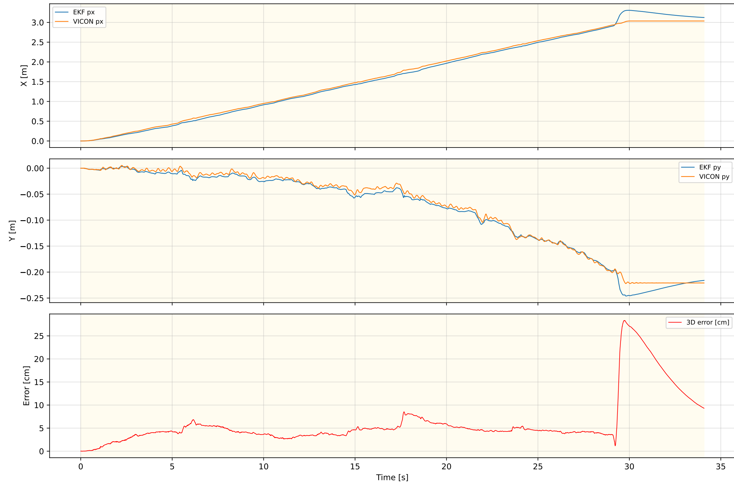
Inner EKF Position — RUGG_WLW_NEW_REAL_1
