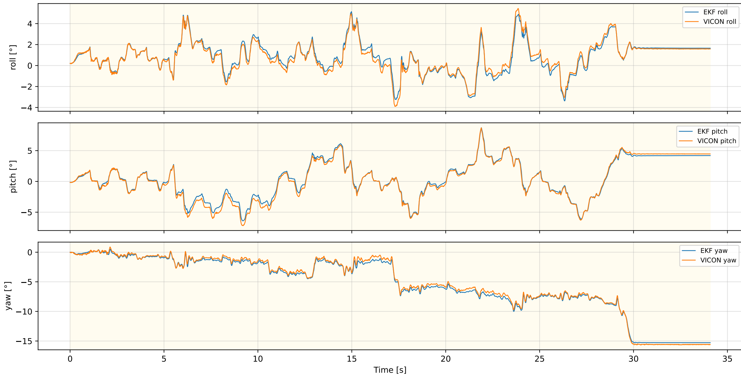
Inner EKF Attitude — RUGG_WLW_NEW_REAL_1
