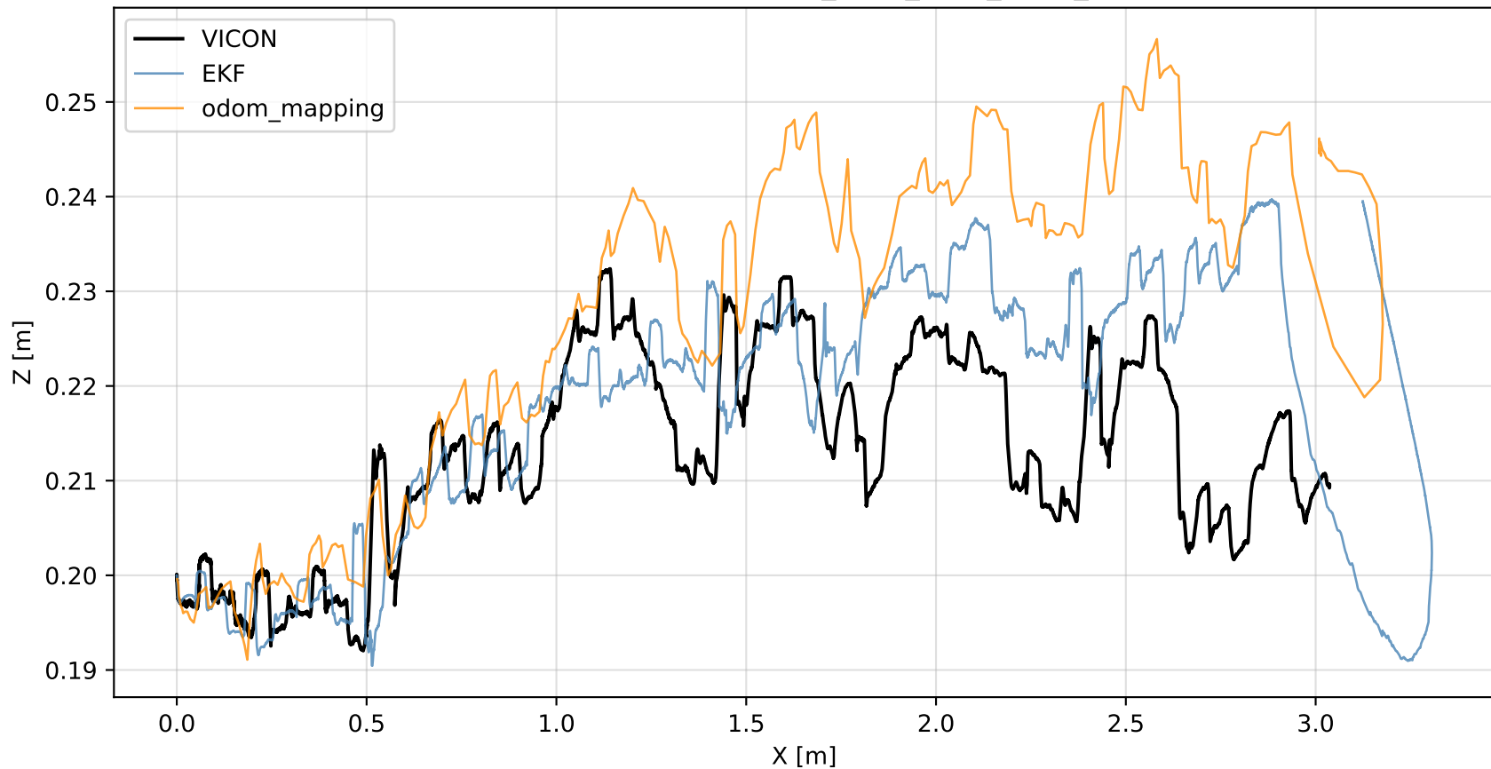
XZ Trajectory — RUGG_WLW_NEW_REAL_1
