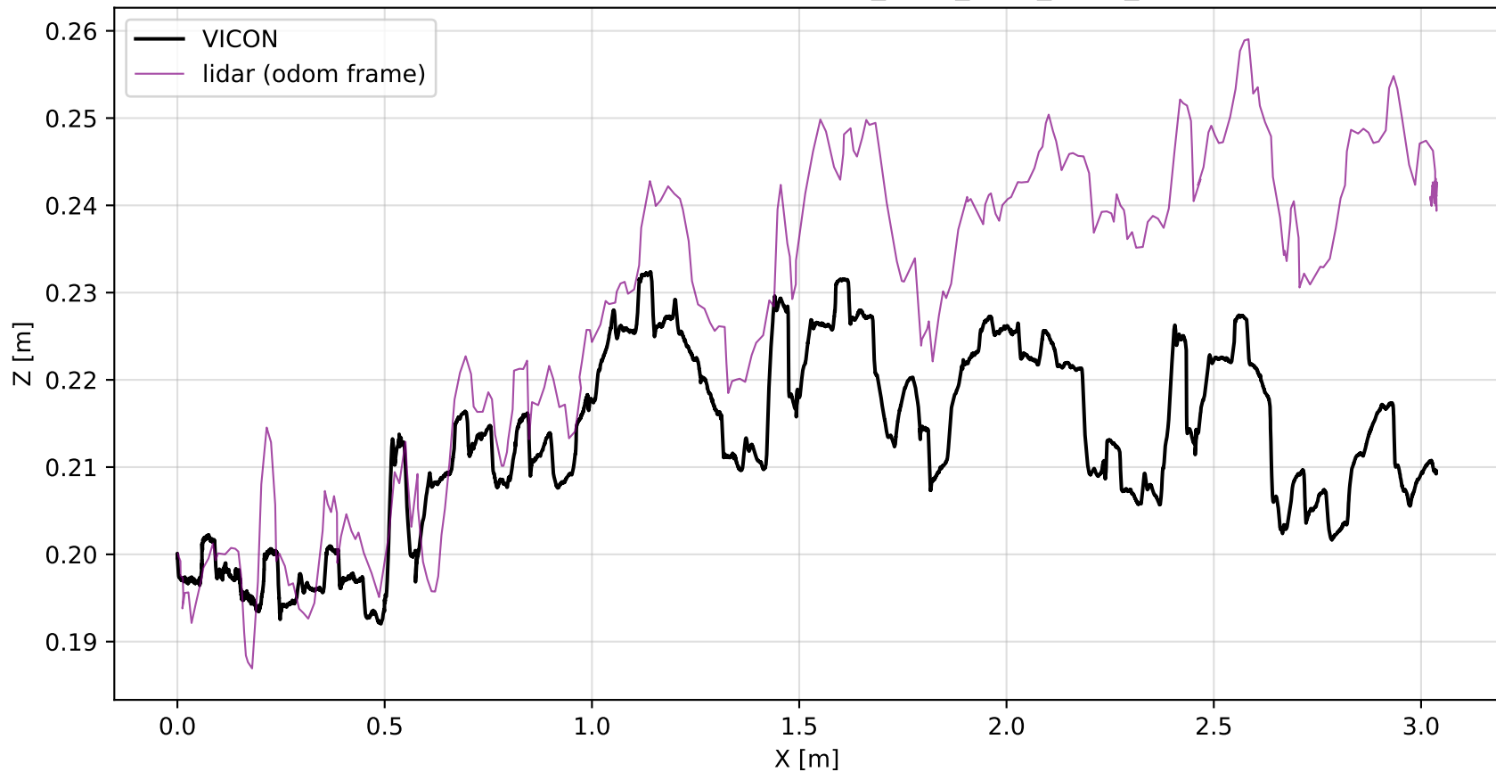
LiDAR XZ Trajectory — RUGG_WLW_NEW_REAL_1
