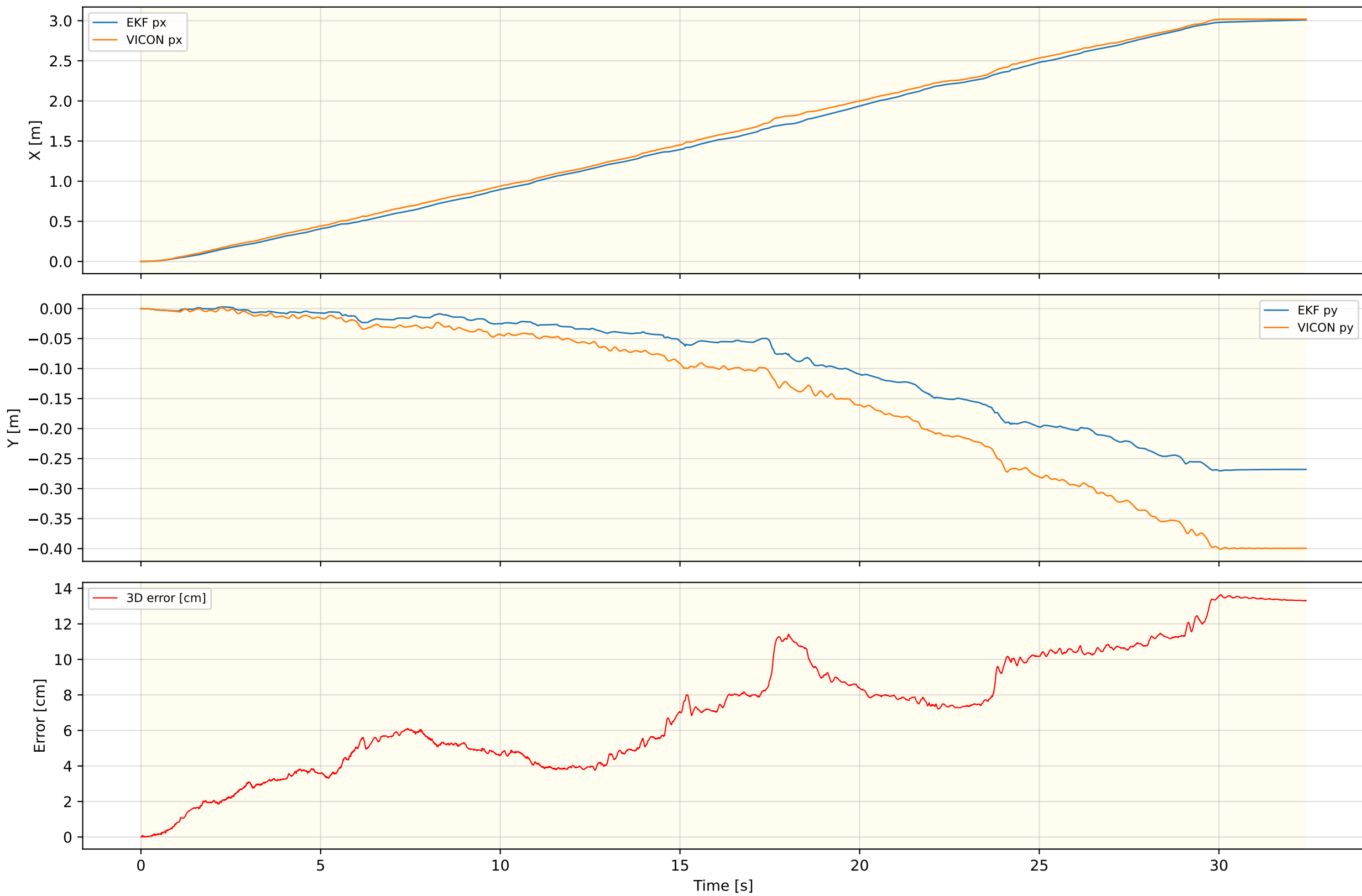
Inner EKF Position — RUGG_WLW_NEW_REAL_2
