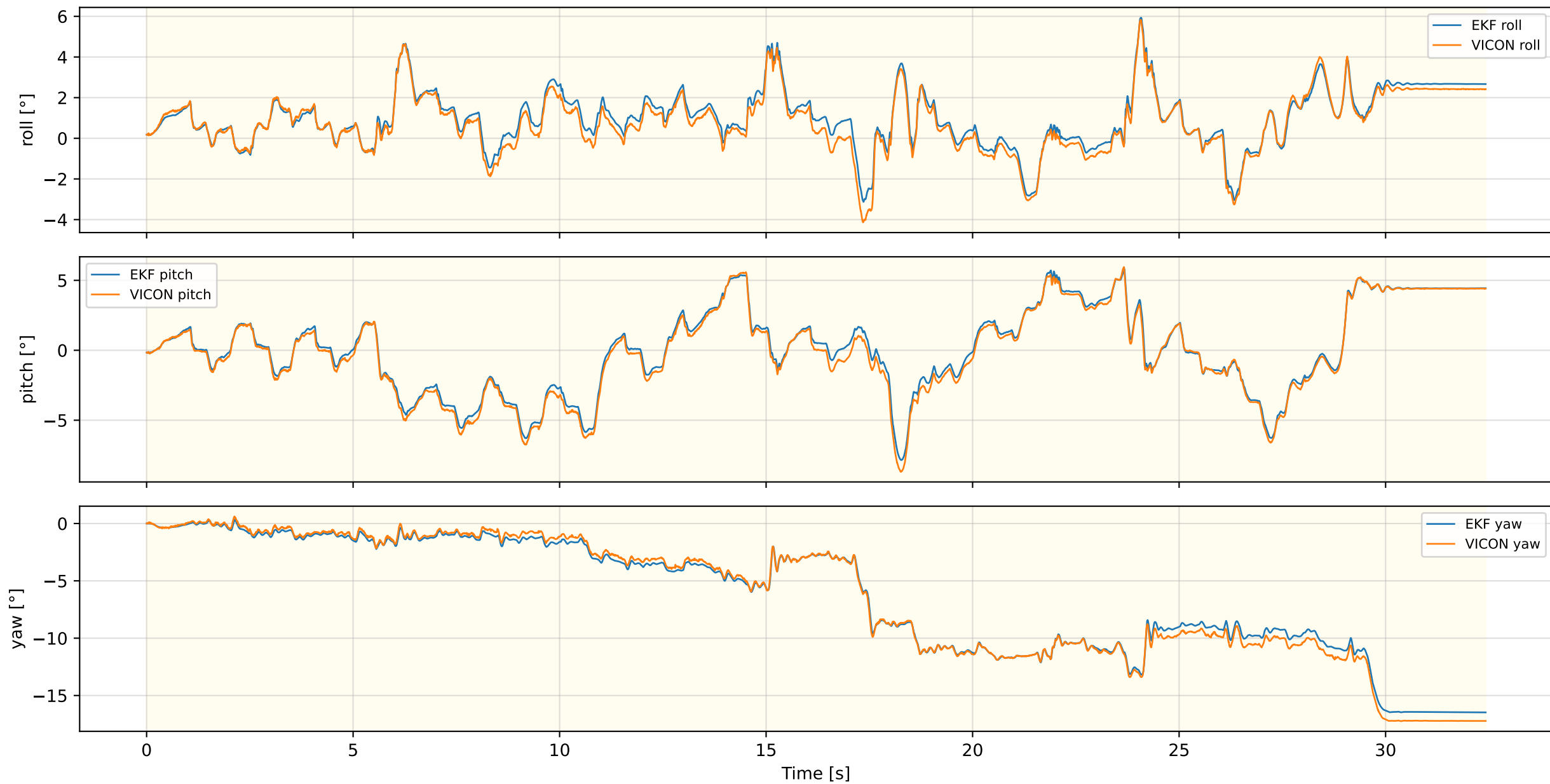
Inner EKF Attitude — RUGG_WLW_NEW_REAL_2
