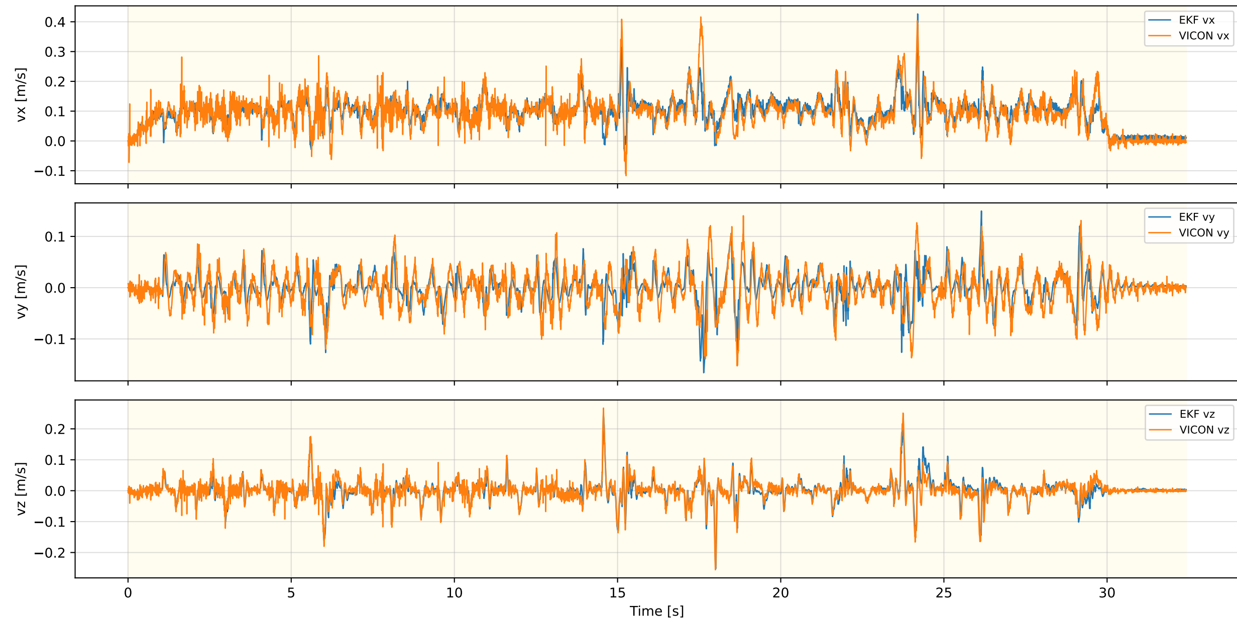
Inner EKF Velocity — RUGG_WLW_NEW_REAL_2
