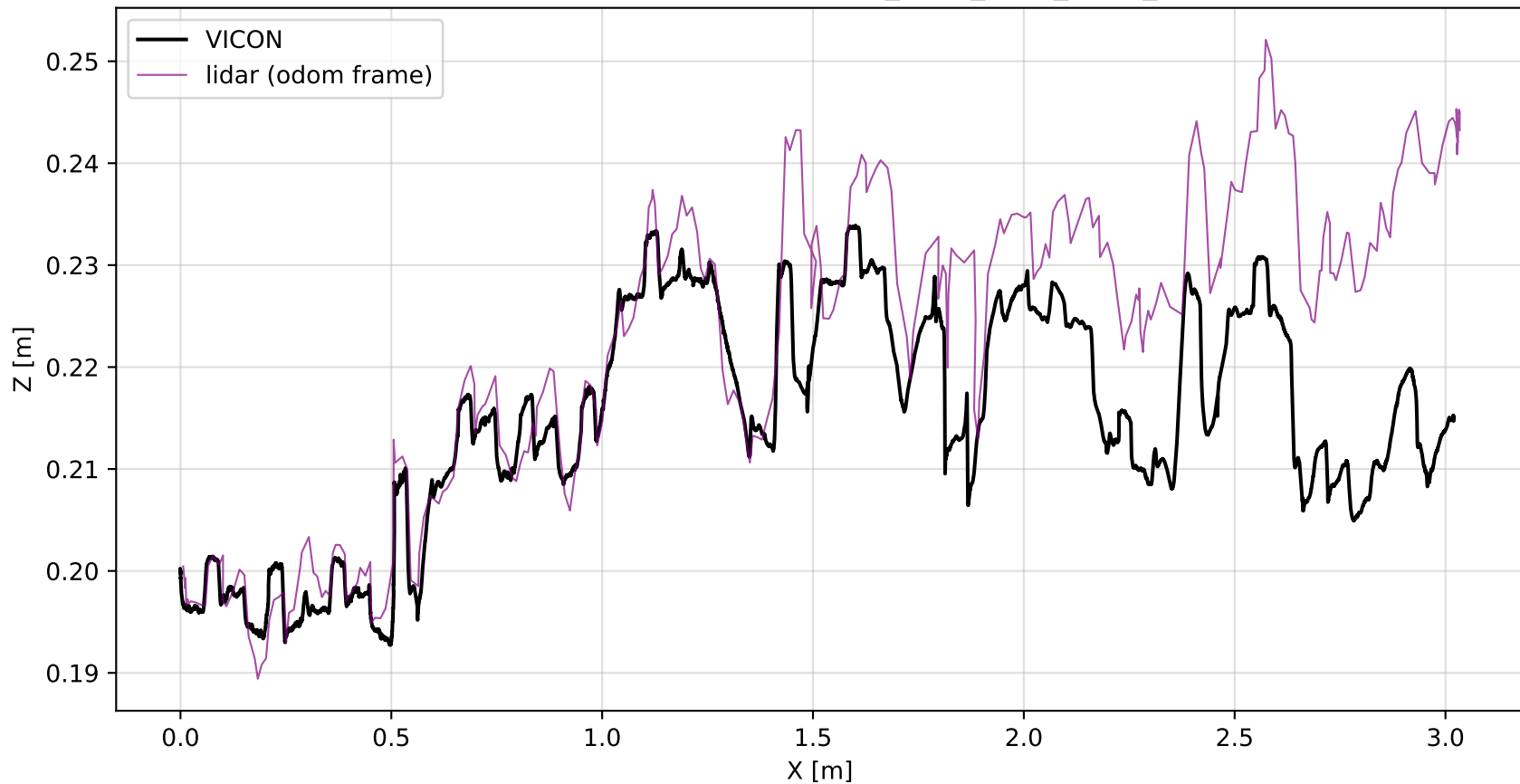
LiDAR XZ Trajectory — RUGG_WLW_NEW_REAL_2
