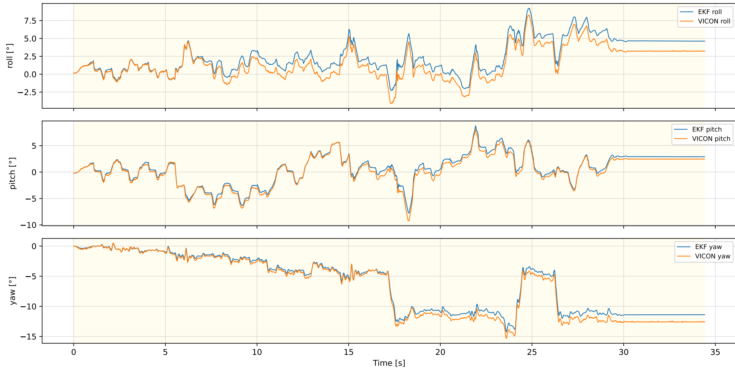
Inner EKF Attitude — RUGG_WLW_NEW_REAL_3
