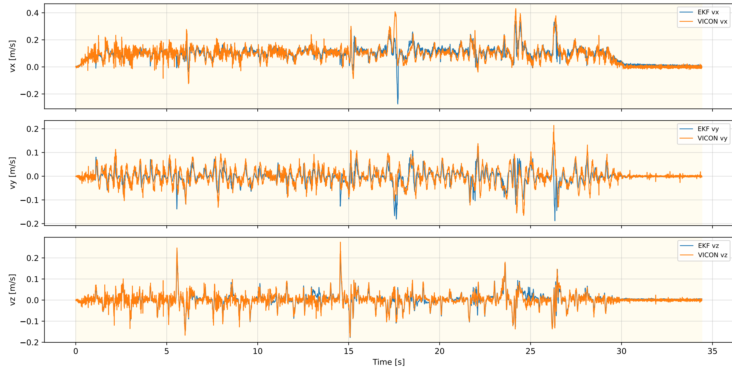
Inner EKF Velocity — RUGG_WLW_NEW_REAL_3
