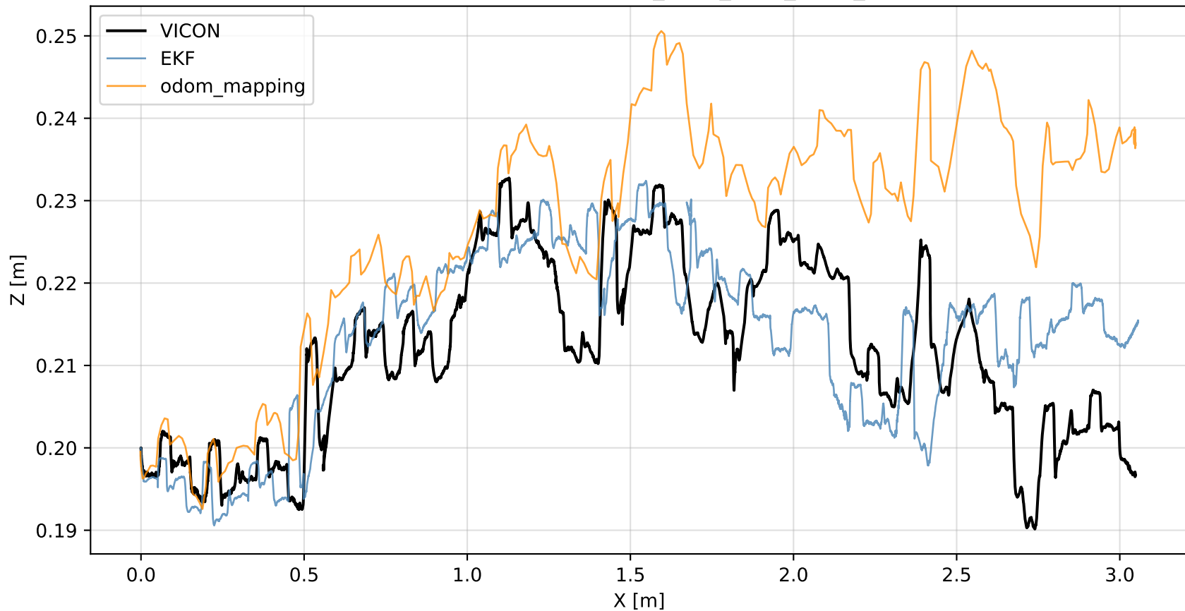
XZ Trajectory — RUGG_WLW_NEW_REAL_3
