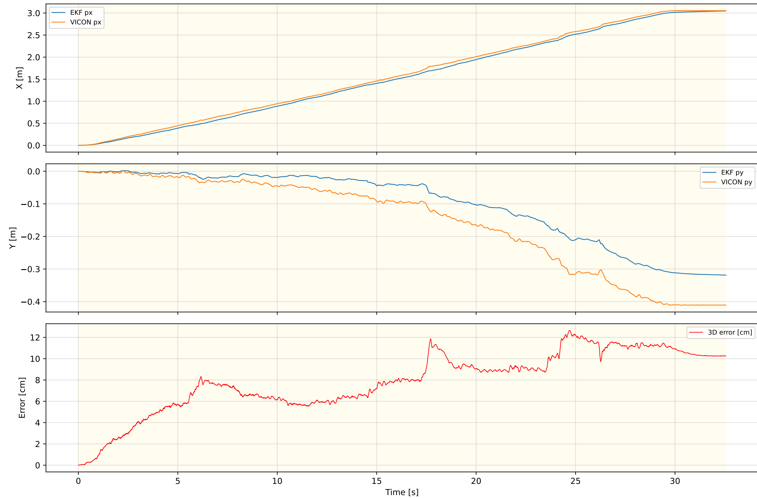
Inner EKF Position — RUGG_WLW_NEW_REAL_4
