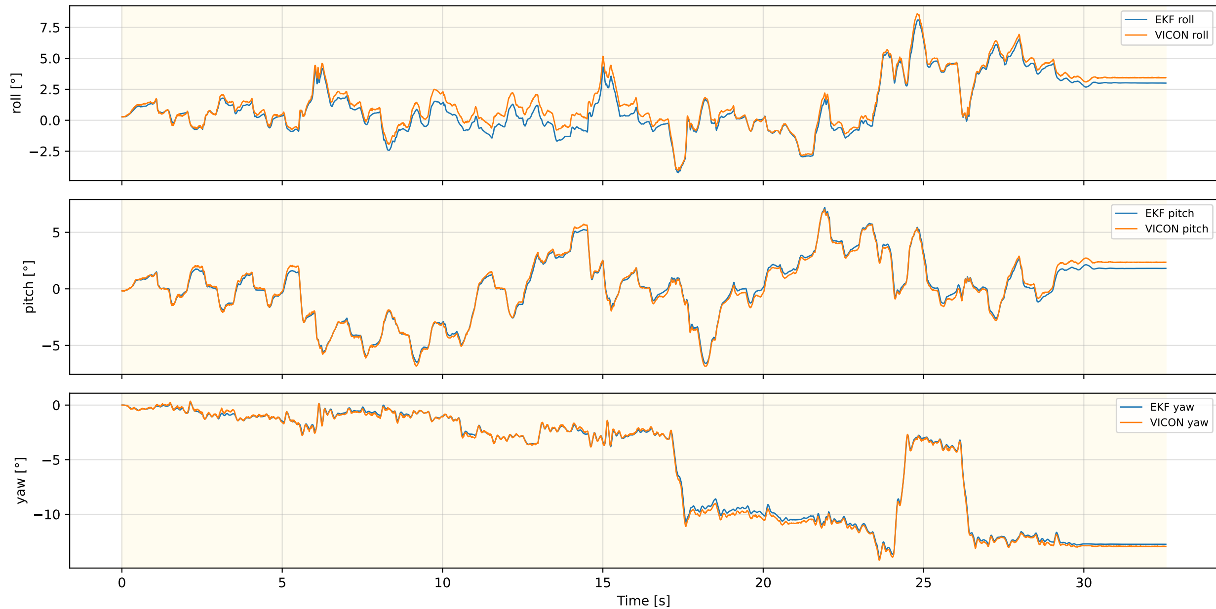
Inner EKF Attitude — RUGG_WLW_NEW_REAL_4
