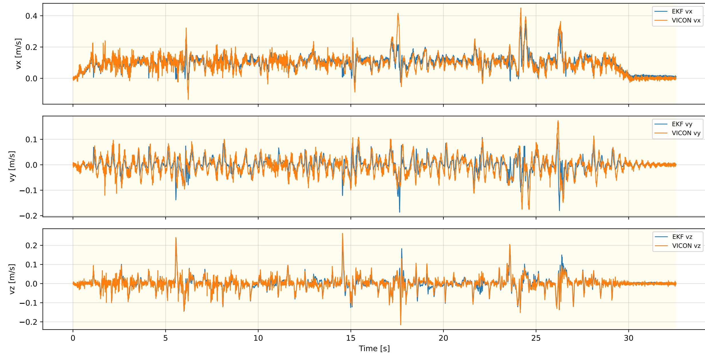
Inner EKF Velocity — RUGG_WLW_NEW_REAL_4
