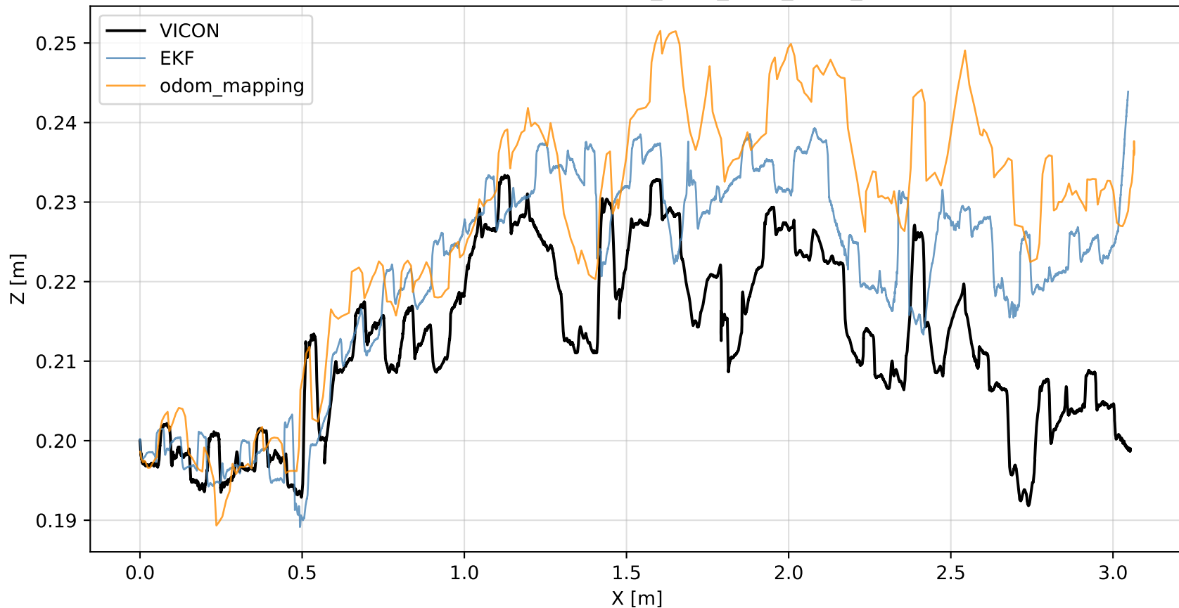
XZ Trajectory — RUGG_WLW_NEW_REAL_4
