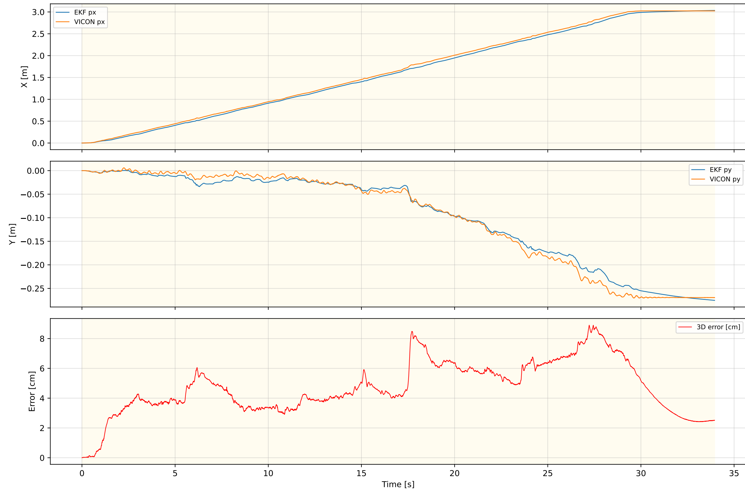
Inner EKF Position — RUGG_WLW_NEW_REAL_5
