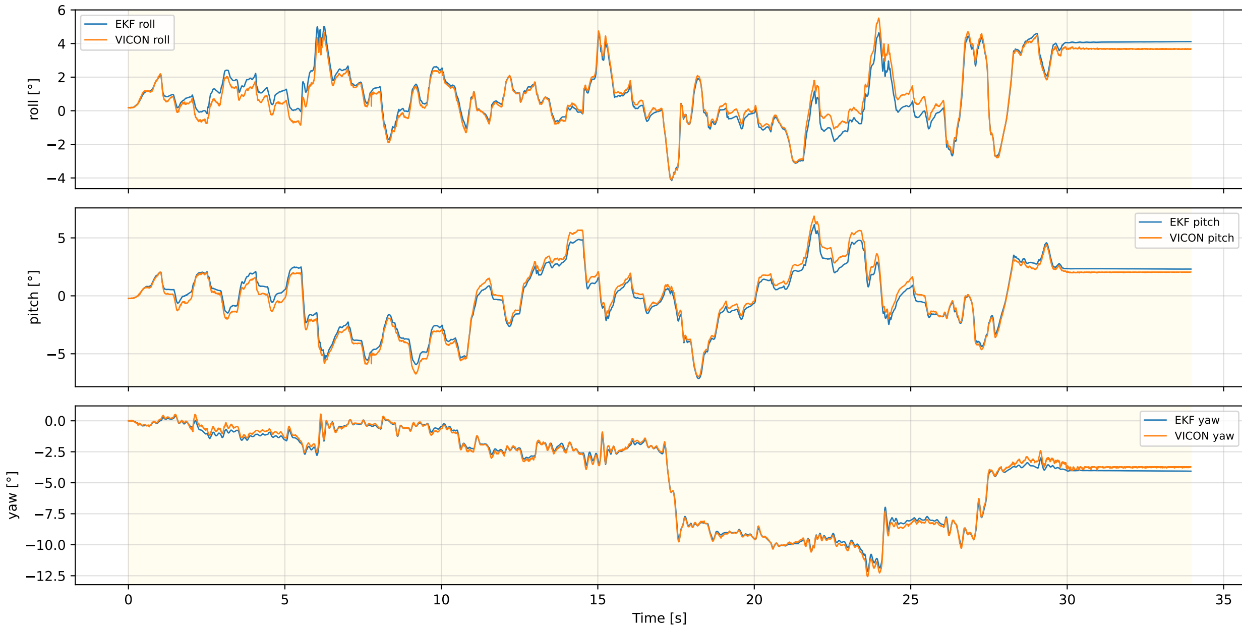
Inner EKF Attitude — RUGG_WLW_NEW_REAL_5
