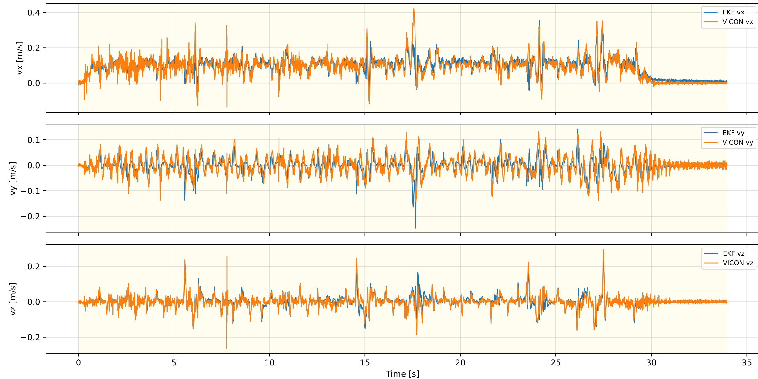
Inner EKF Velocity — RUGG_WLW_NEW_REAL_5
