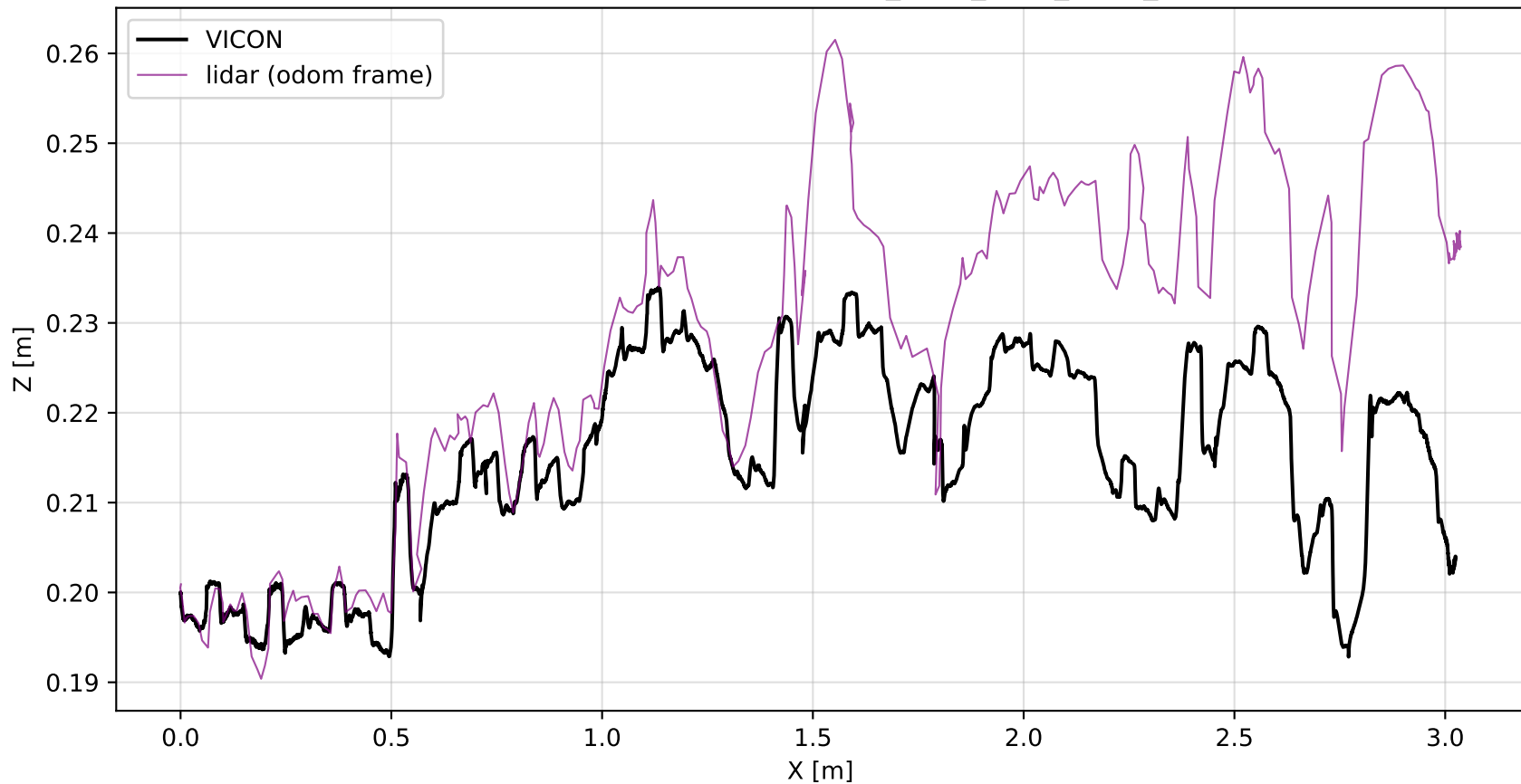
LiDAR XZ Trajectory — RUGG_WLW_NEW_REAL_5
